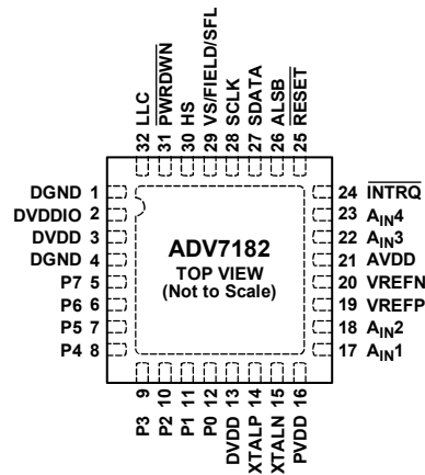
Figure 4. Pin Configuration
