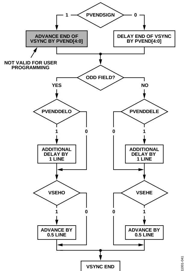
Figure 40. PAL VSYNC End
