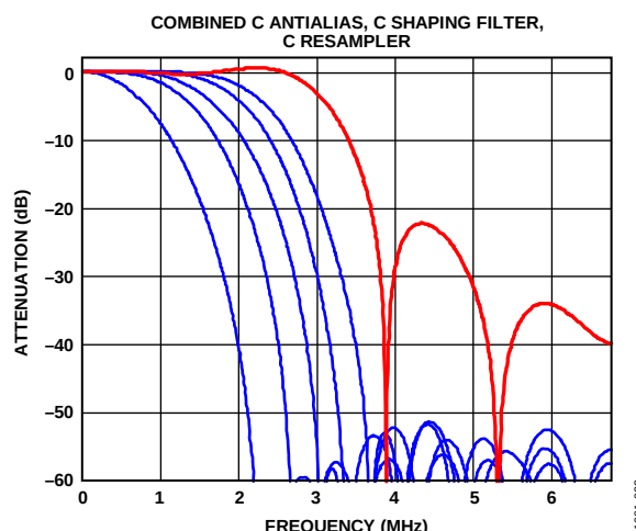
Figure 22. Chroma Shaping Filter Responses
