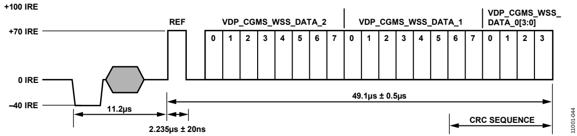
Figure 43. CGMS Waveform
