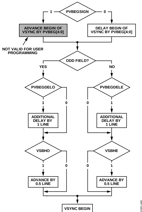
Figure 39. PAL VSYNC Begin
