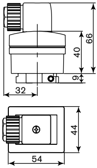
Mounted on S030 fitting
