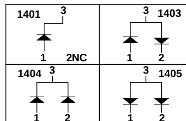
Connection Diagrams
