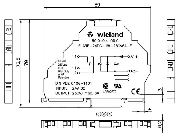
Dimensional diagram
