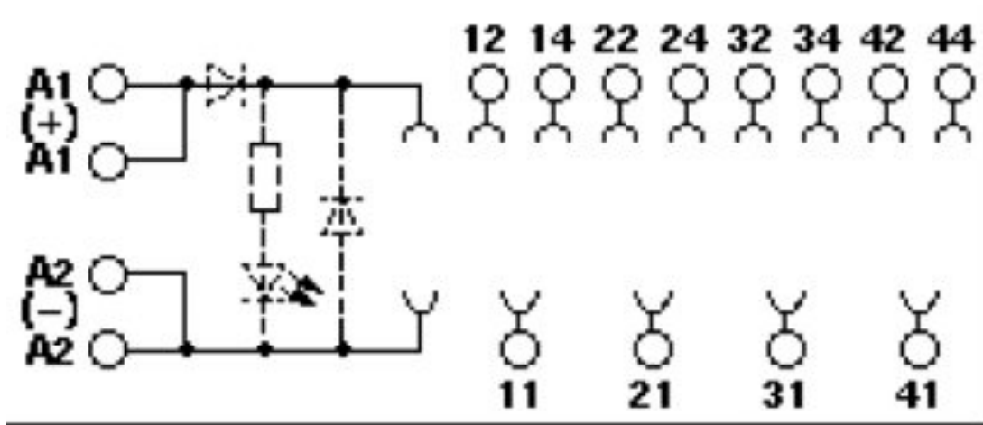
Circuit diagram
