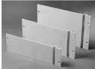
Rack mount adapter kits for ½ MW (5063-9240 (34190A), 5063-9243 (34193A), 5063-9245)
