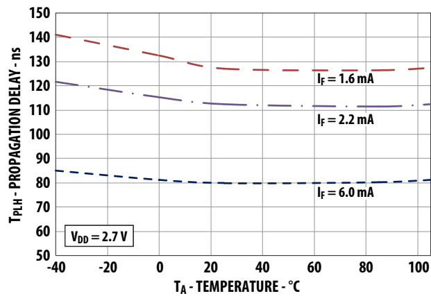
Figure 9. Propagation Delay, t_{PL} vs. Temperature
