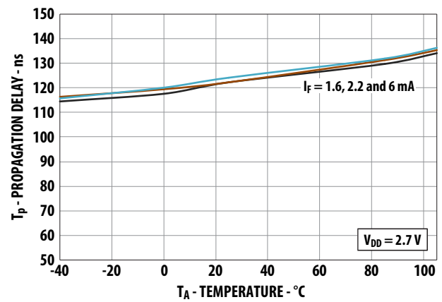
Figure 8. Propagation Delay, t_{PL} vs. Temperature
