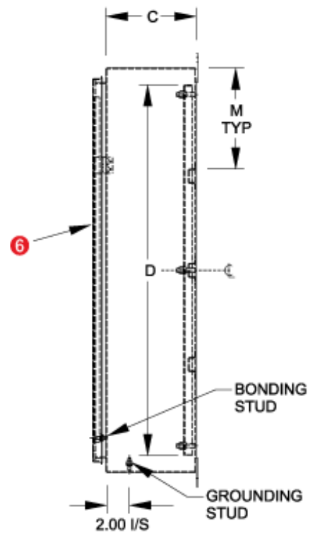
Formed View
