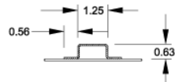
Section Z-Z
