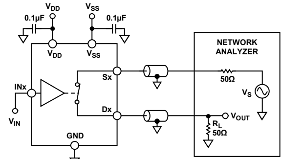
Figure 29. Bandwidth
