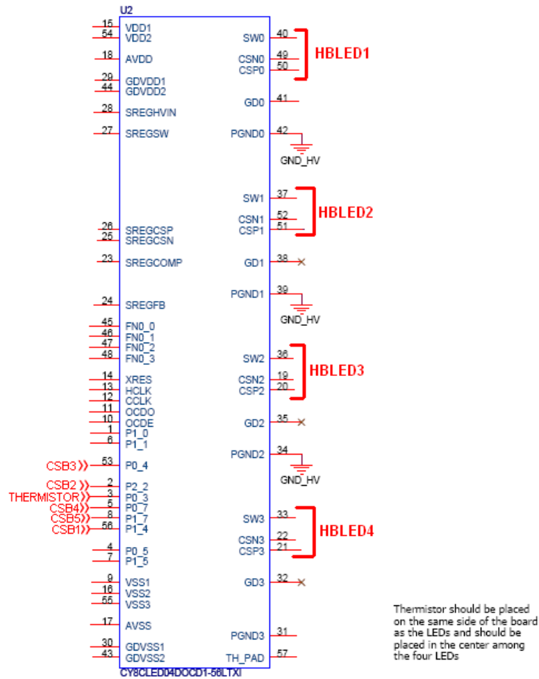
Figure 4-5. PowerPSoC Connections
