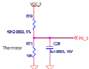
Figure 4-11. Thermistor Circuit
