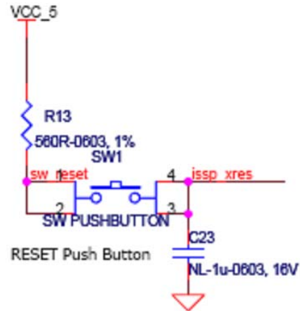
Figure 4-9. RESET Circuit
