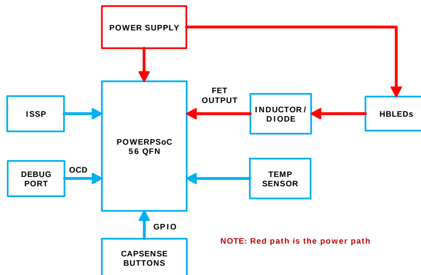
Figure 4-1. Block Diagram
