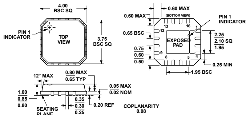
Figure 51. 16-Lead Lead Frame Chip Scale Package [LFCSP_VQ] 4 mm × 4 mm Body, Very Thin Quad (CP-16-4)
