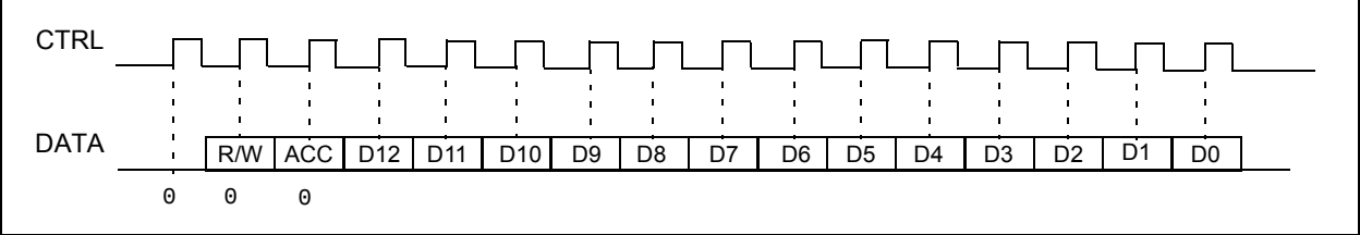
FIGURE 9-3: CONFIGURATION REGISTER 'WRITE'
