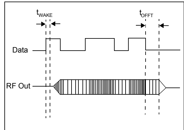
FIGURE 9-2: TRANSMITTER TIMING IN PRESET MODE
