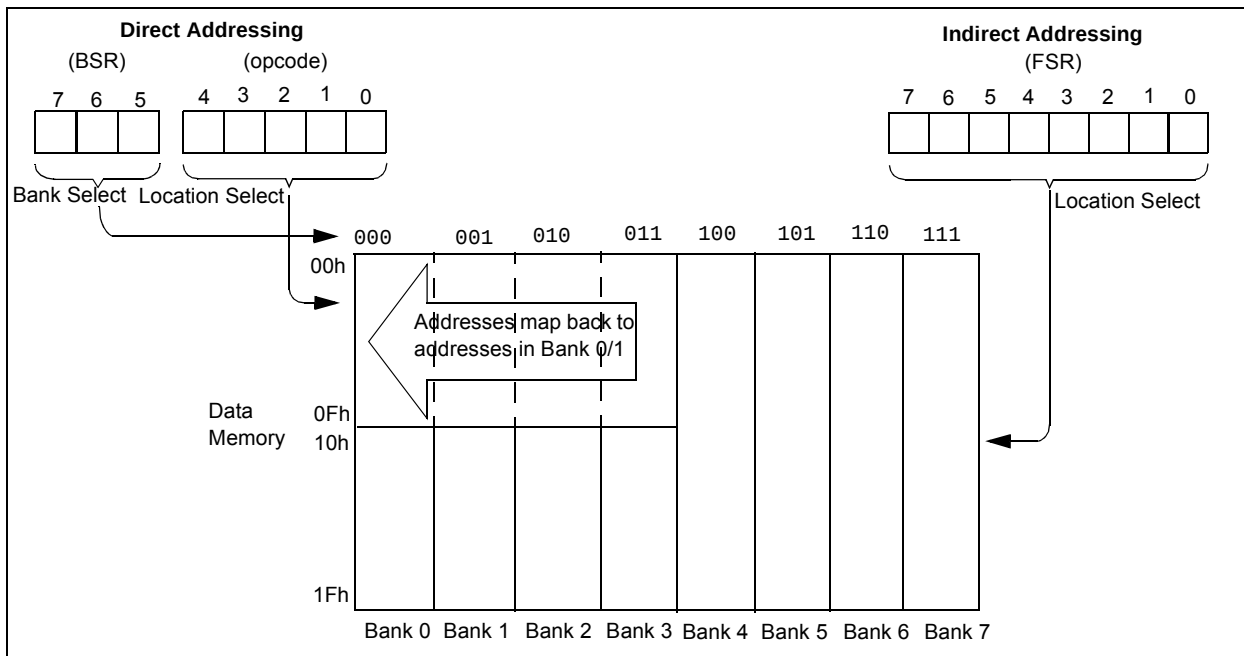
FIGURE 4-4: DIRECT/INDIRECT ADDRESSING
