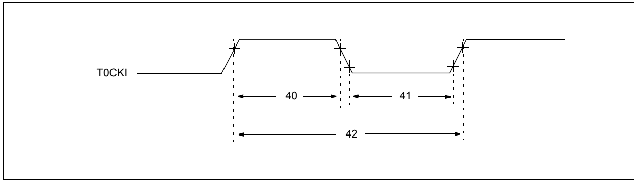
FIGURE 12-7: TIMER0 CLOCK TIMINGS
