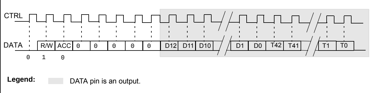
FIGURE 9-4: CONFIGURATION REGISTER 'READ'
