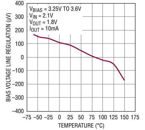
Bias Voltage Line Regulation
