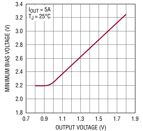
Minimum BIAS Voltage vs VOUT
