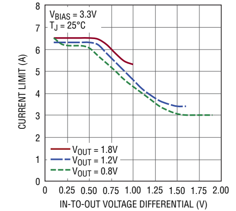
Current Limit vs V_{IN} - V_{OUT}
