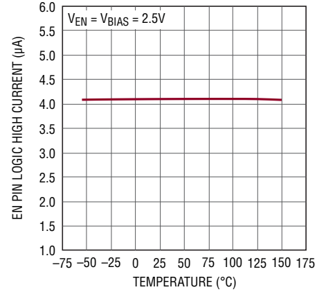
EN Pin Logic High Current
