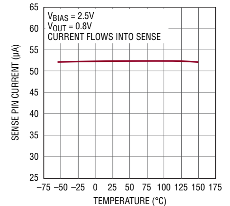
SENSE Pin Current
