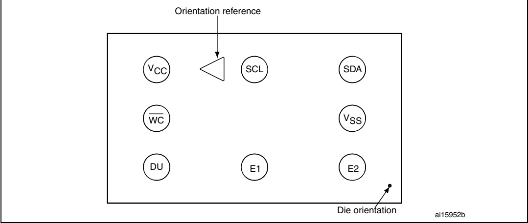
Figure 3. WLCSP8 connections
