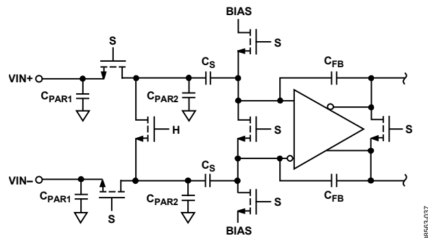
Figure 29. Switched-Capacitor Input
