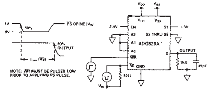
Test Circuit 10. Reset Turn-Off Time, t_{OFF}(\overline{RS})
