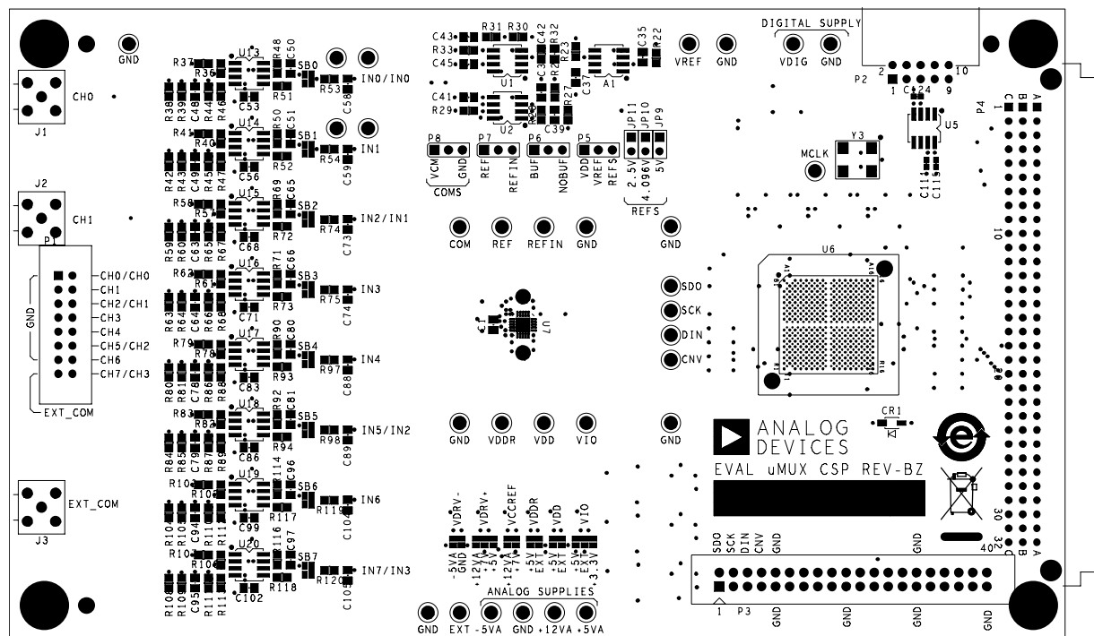
Figure 20. Top Side Silk-Screen
