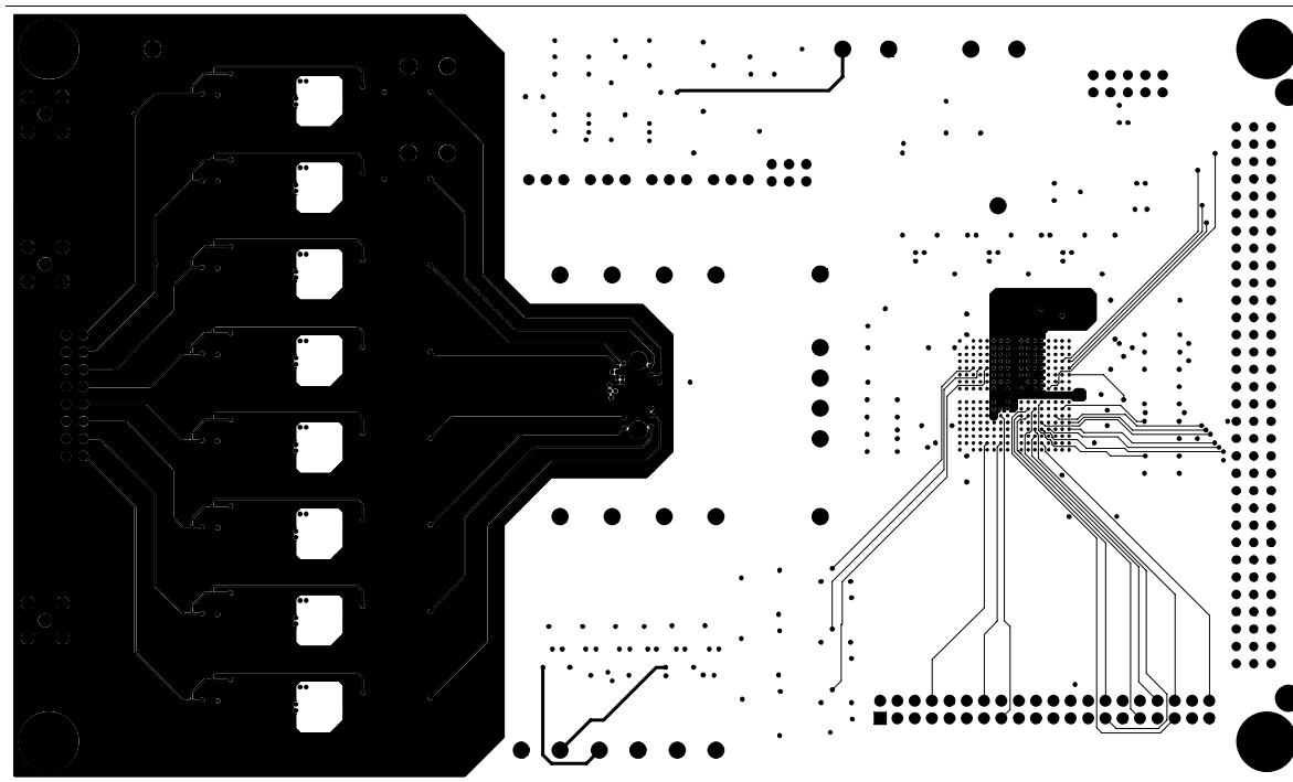
Figure 21. Inner Layer 1
