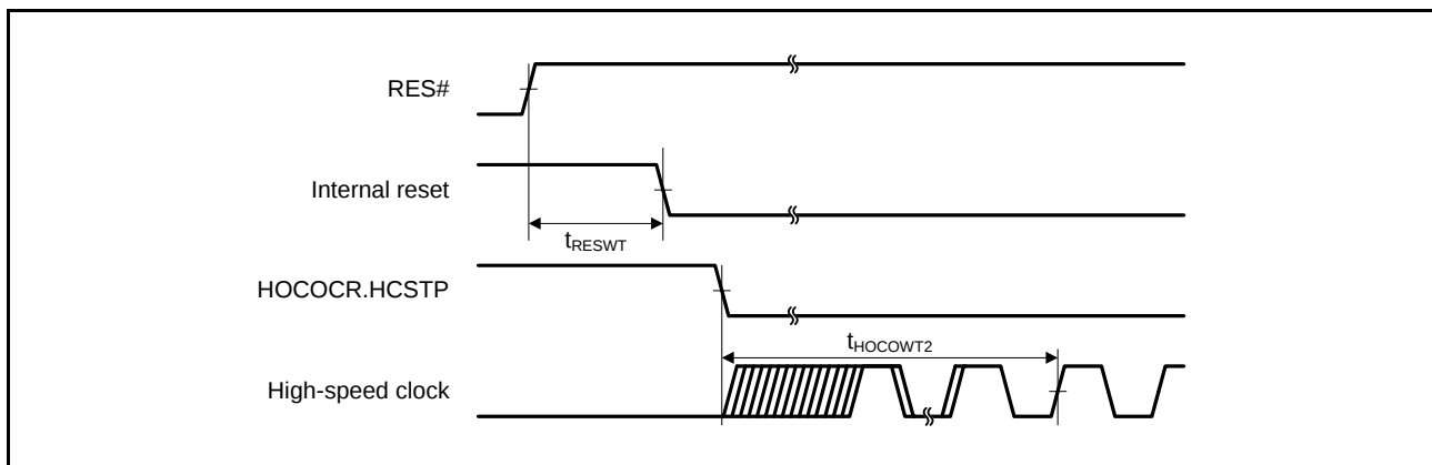
Figure 5.6 High-Speed Clock Oscillation Start Timing (Oscillation is Started by Setting the HOCOCCR.HCSTP Bit)
