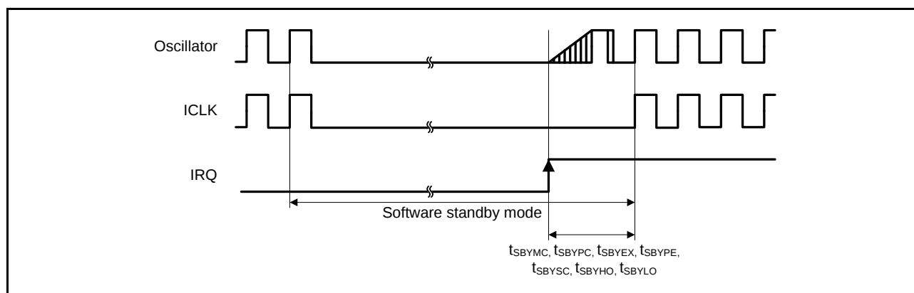
Figure 5.14 Software Standby Mode Cancellation Timing
