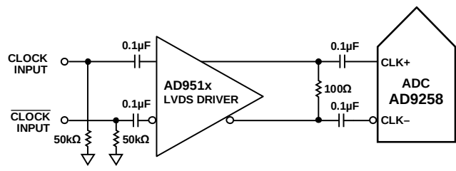
Figure 78. Differential LVDS Sample Clock (Up to 625 MHz)
