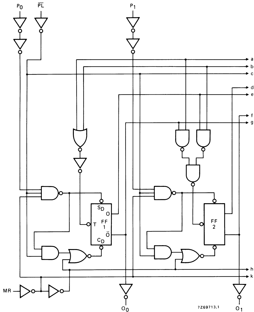
Fig.3 Logic diagram (continued on Fig.4).
