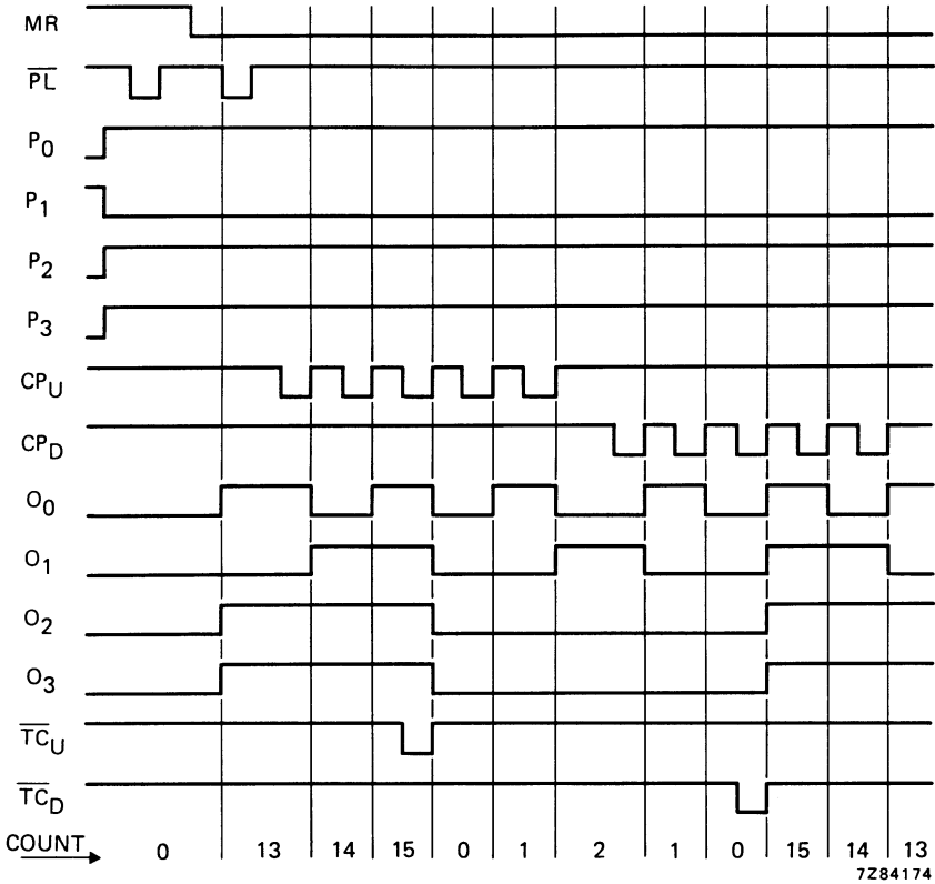
Fig.7 Timing diagram.
