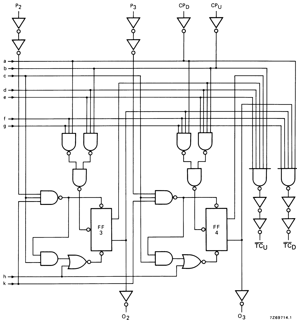
Fig.4 Logic diagram (continued from Fig.3).
