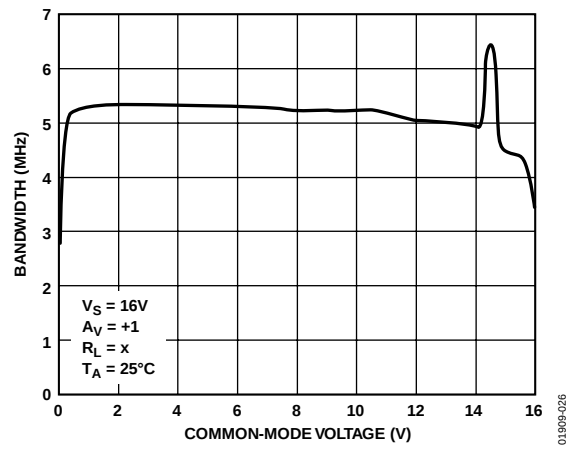
Figure 26. Frequency vs. Common-Mode Voltage ( V_S = 16\text{ V} )
