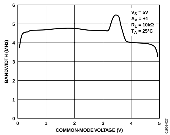
Figure 27. Frequency vs. Common-Mode Voltage ( V_S = 5\text{ V} )
