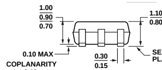
Figure 35. 5-Lead Thin Shrink Small Outline Transistor Package [SC70] (KS-5)
