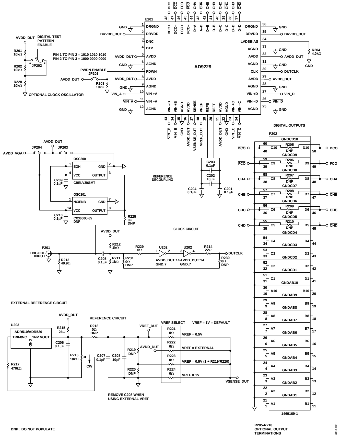
Figure 49. Evaluation Board Schematic, DUT, VREF, Clock Inputs, and Digital Output Interface
