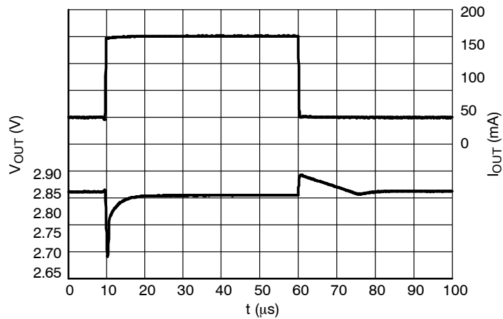
Figure 34. Load Transients, 2.8 V Version, I_{OUT} = 1 - 150 \text{ mA} , t_R = t_F = 0.5 \mu s , V_{IN} = 3.8 \text{ V}
