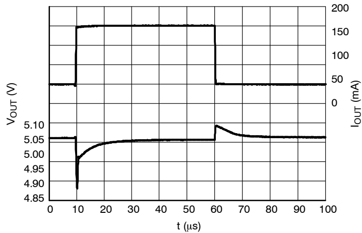
Figure 35. Load Transients, 5.0 V Version, I_{OUT} = 1 - 150 \text{ mA} , t_R = t_F = 0.5 \mu s , V_{IN} = 6.0 \text{ V}
