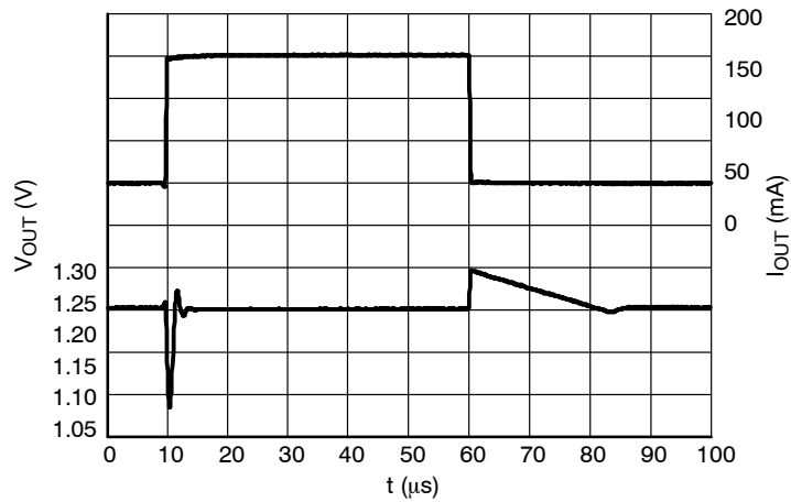
Figure 33. Load Transients, 1.2 V Version, I_{OUT} = 1 - 150 \text{ mA} , t_R = t_F = 0.5 \mu s , V_{IN} = 2.2 \text{ V}
