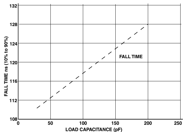
Figure 82. Typical Fall Time (10% to 90%) vs. Load Capacitance for Driver E at V_{DDEXT} = 2.7 V
