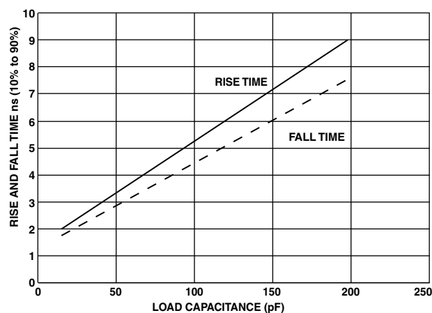
Figure 75. Typical Rise and Fall Times (10% to 90%) vs. Load Capacitance for Driver B at V_{DDEXT} = 3.65\text{ V}
