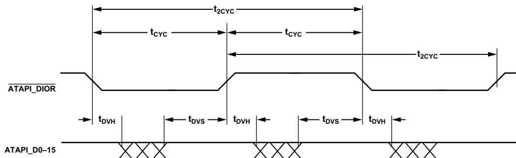
Figure 55. Sustained Ultra DMA Data-Out Burst 1
