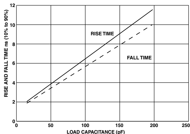
Figure 73. Typical Rise and Fall Times (10% to 90%) vs. Load Capacitance for Driver A at V_{DDEXT} = 3.65\text{ V}
