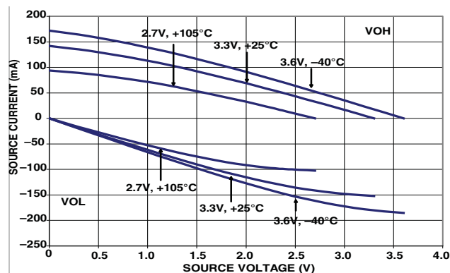
Figure 62. Drive Current B (High V_{DDEXT} )
