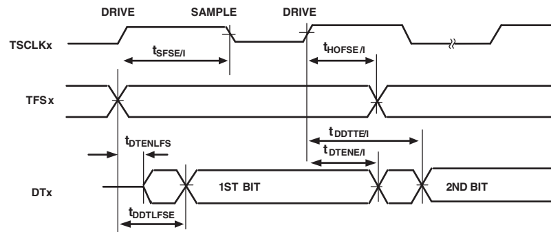
Figure 34. External Late Frame Sync
