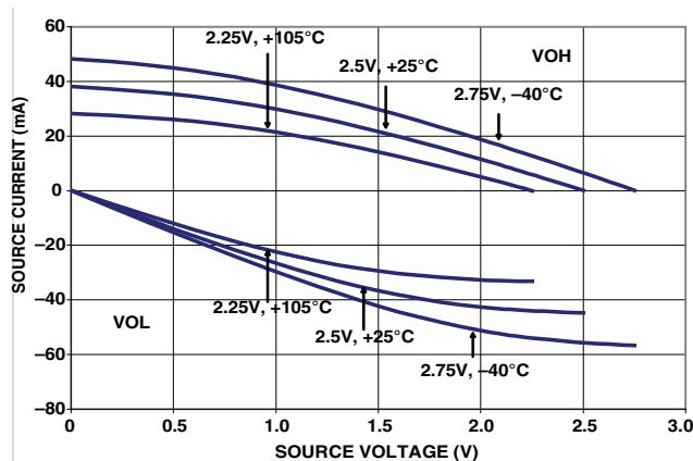
Figure 63. Drive Current C (Low V_{DDEXT} )
