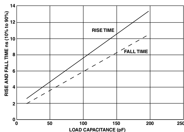
Figure 72. Typical Rise and Fall Times (10% to 90%) vs. Load Capacitance for Driver A at V_{DDEXT} = 2.25\text{ V}
