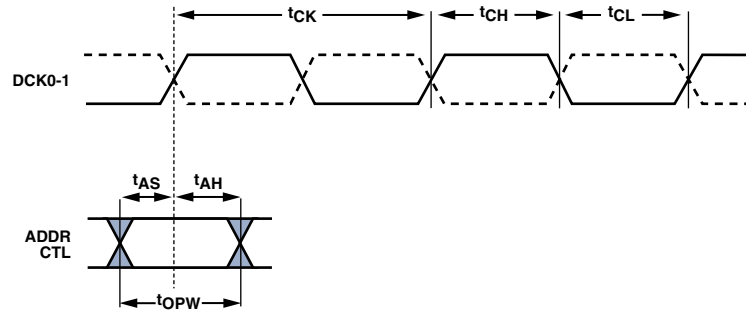
Figure 16. DDR SDRAM /Mobile DDR SDRAM Clock and Control Cycle Timing
