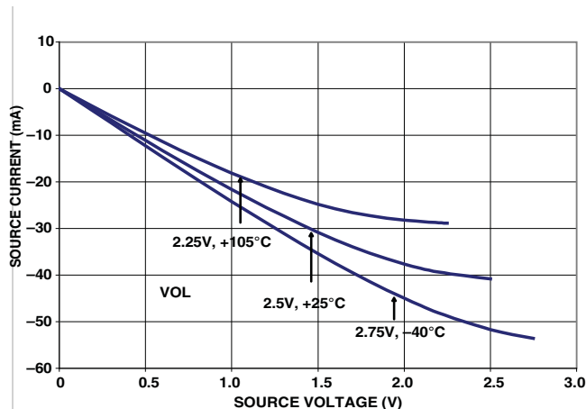
Figure 67. Drive Current E (Low V_{DDEXT} )
