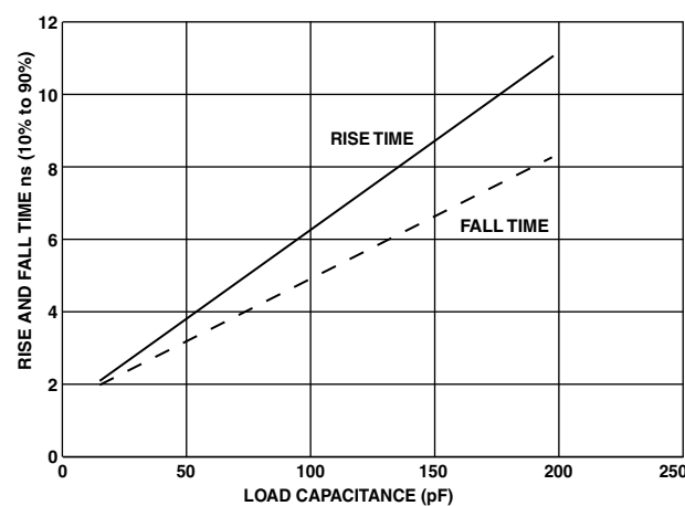
Figure 74. Typical Rise and Fall Times (10% to 90%) vs. Load Capacitance for Driver B at V_{DDEXT} = 2.25\text{ V}
