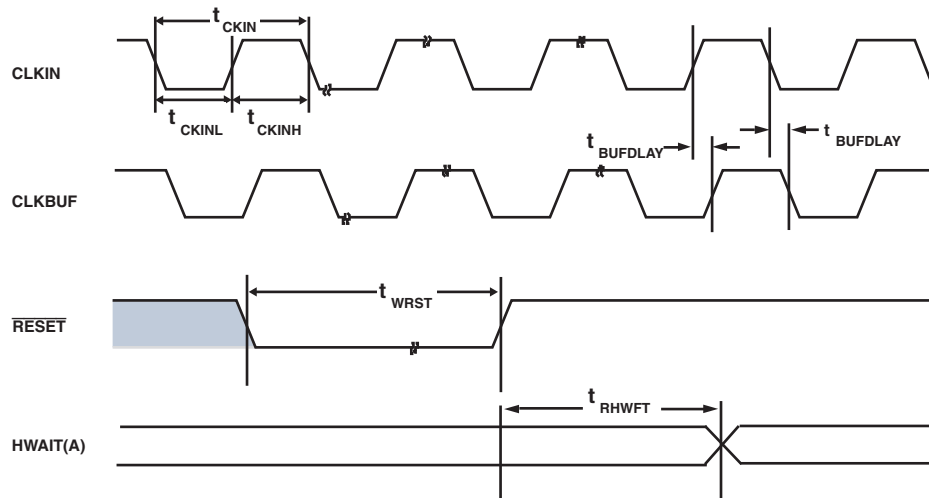
Figure 10. Clock and Reset Timing
