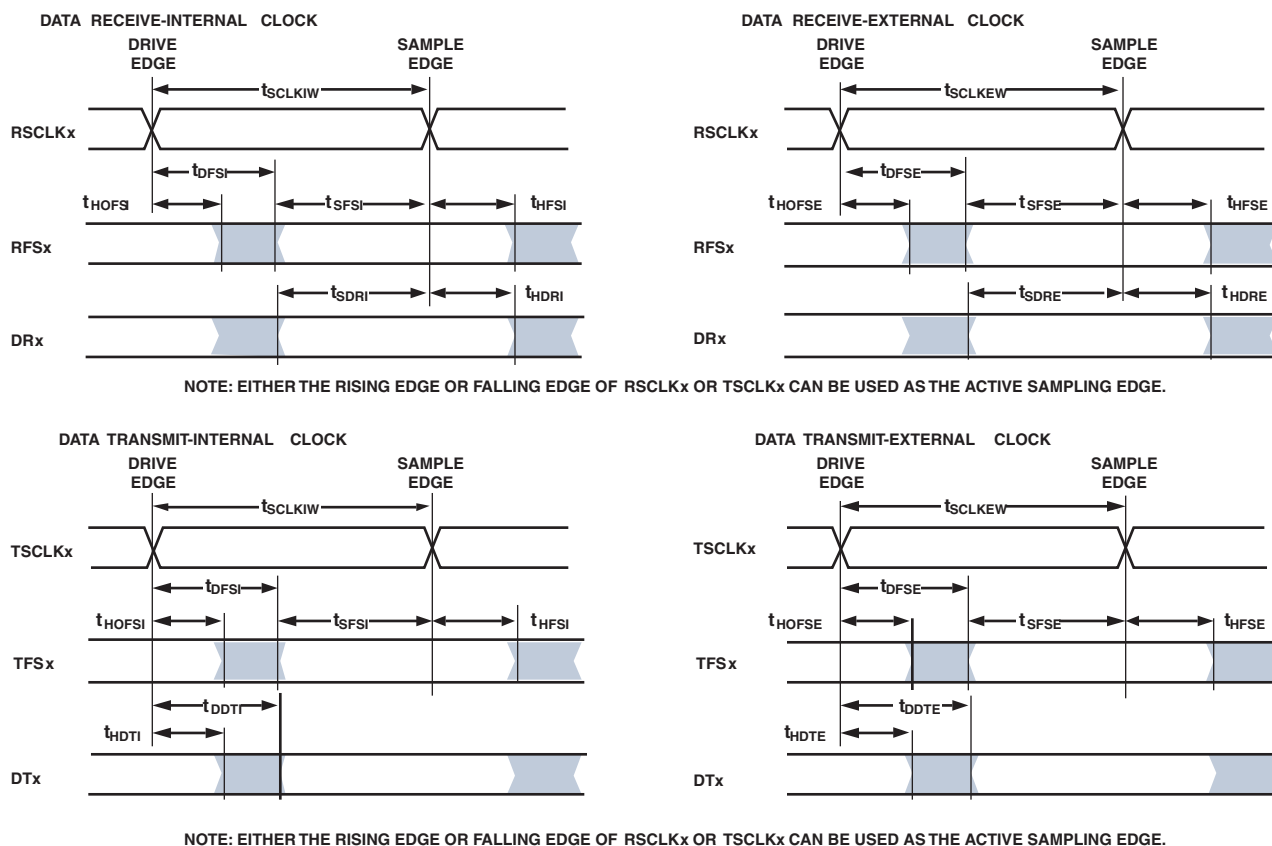
Figure 33. Serial Ports
