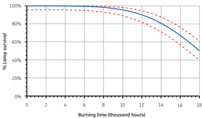
CMH G8.5 35W 4200K
