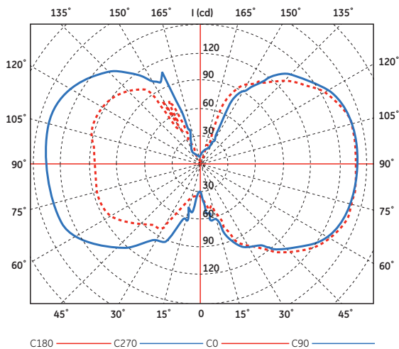
Vertical plane polar intensity curve I_{max}=170.13 cd at 100^\circ
