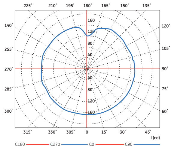
Horizontal plane polar intensity curve I_{max}=170.13 cd at 100^\circ
