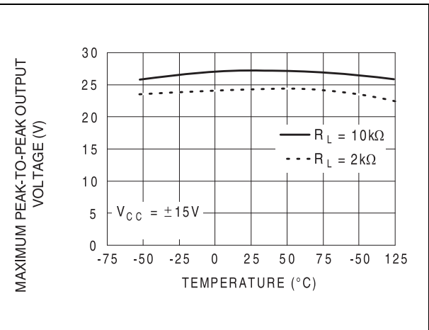
Figure 5. Maximum peak-to-peak output voltage versus free air temperature
