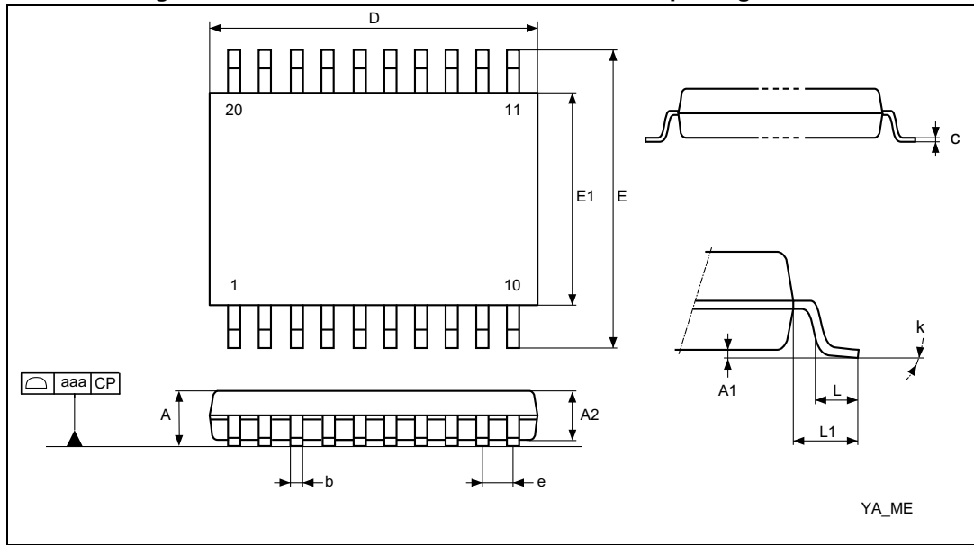
Figure 45. TSSOP20 - 20-lead thin shrink small package outline
