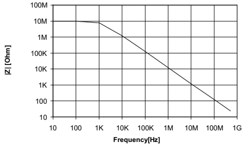
Typical input impedance PMT221A (switched to 10:1)
