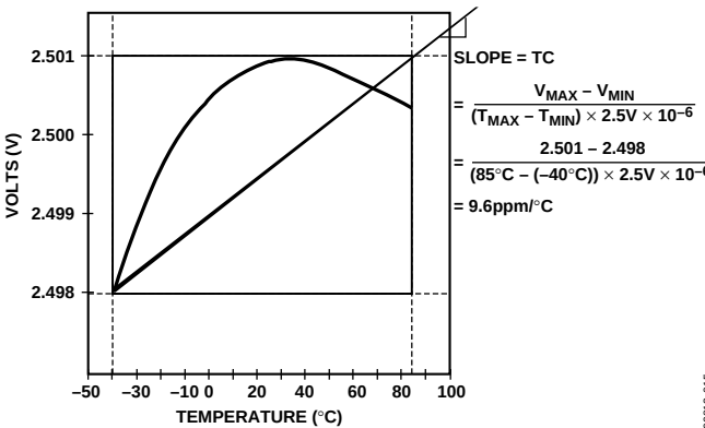
Figure 15. Typical AD680AN/AD680AR Temperature Drift
