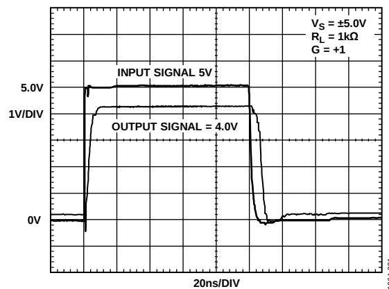
Figure 29. Output Overload Recovery, V_S = \pm 5.0 V
