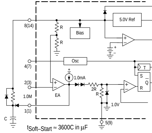
Figure 20. Soft-Start Circuit
