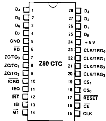
28-Lead DIP Pin Assignments
