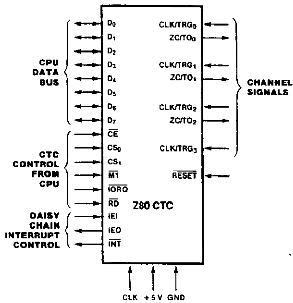
Pin Functions
