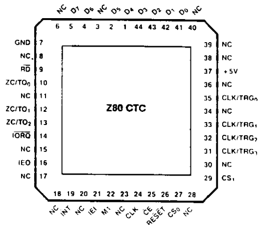
44-Lead PLCC Pin Assignments
