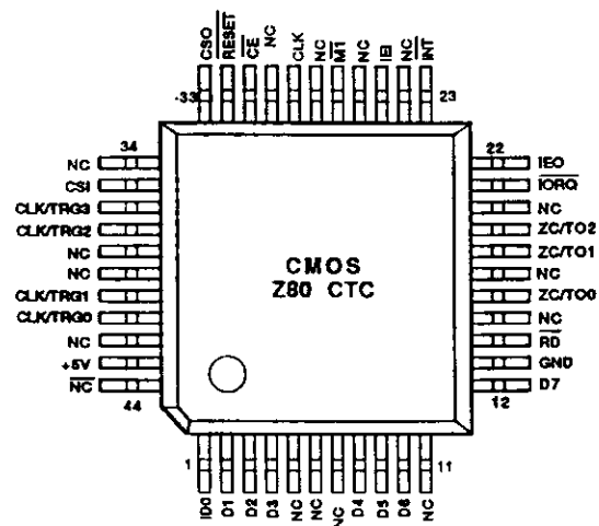
44-Lead QFP Pin Assignments (CMOS Device Only)
