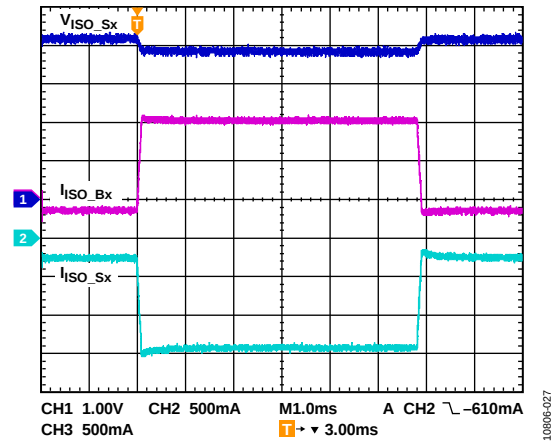
Figure 27. Load Transient, I_{ISO\_Sx} Load = 300 mA to 1500 mA to 300 mA, EN\_CHG = High , ILIM[3:0] = 0110 (Binary) = 500 mA
