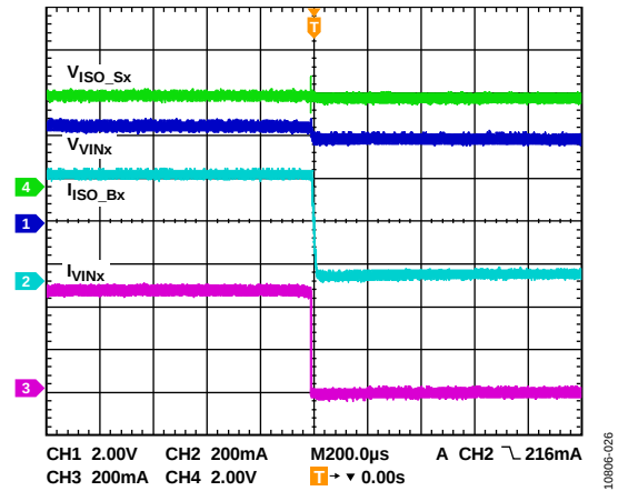
Figure 26. USB VBUS Disconnect
