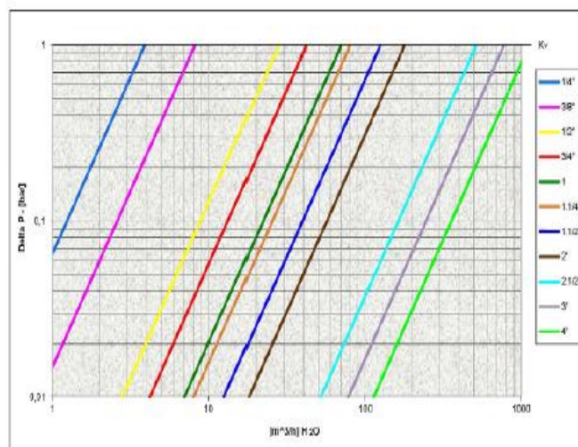
Pressure Drop Chart
