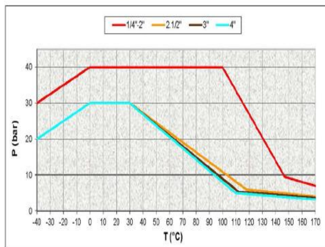
Pressure-Temperature Chart
