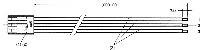
EE-1005 Connector
