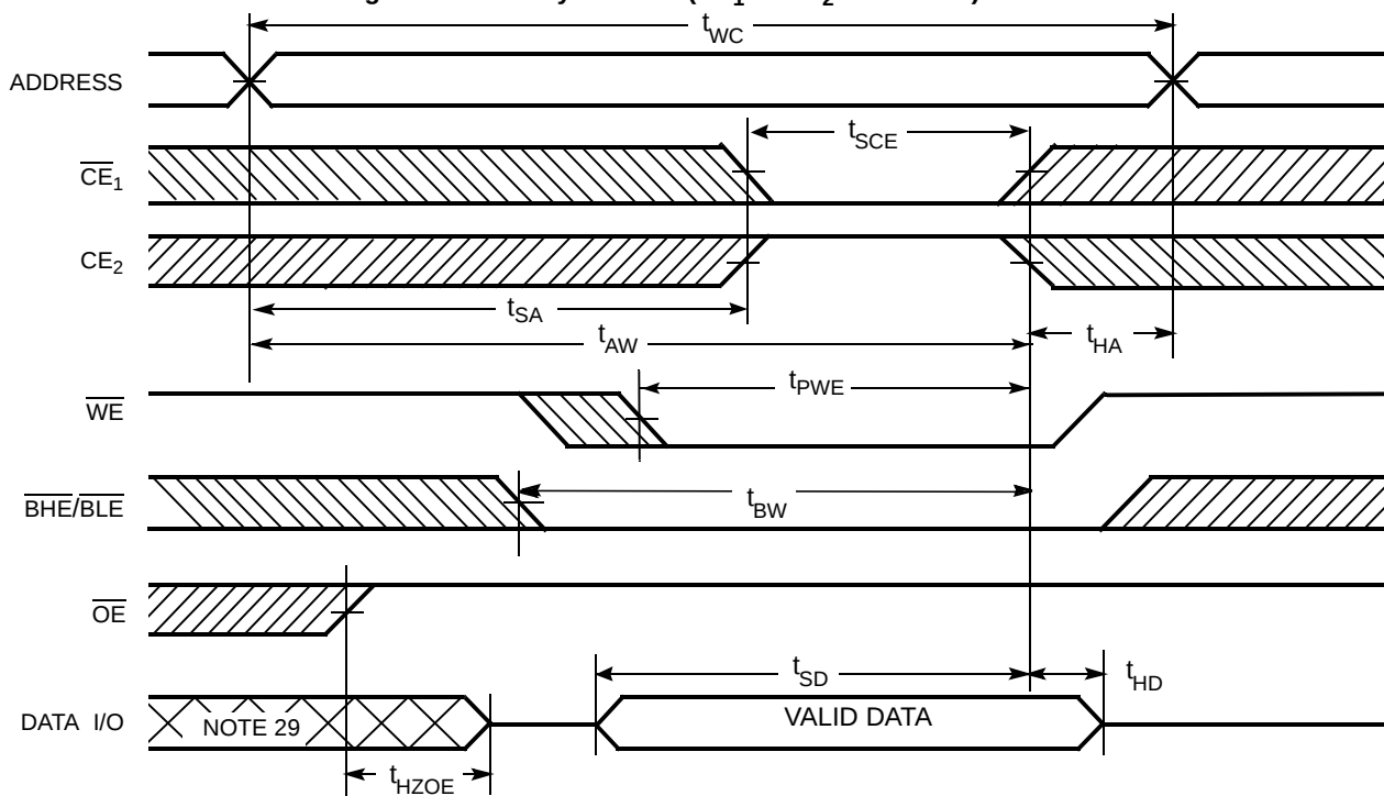
Figure 8. Write Cycle No. 2 ( \overline{\text{CE}}_1 or \text{CE}_2 Controlled) [26, 27, 28, 29]
