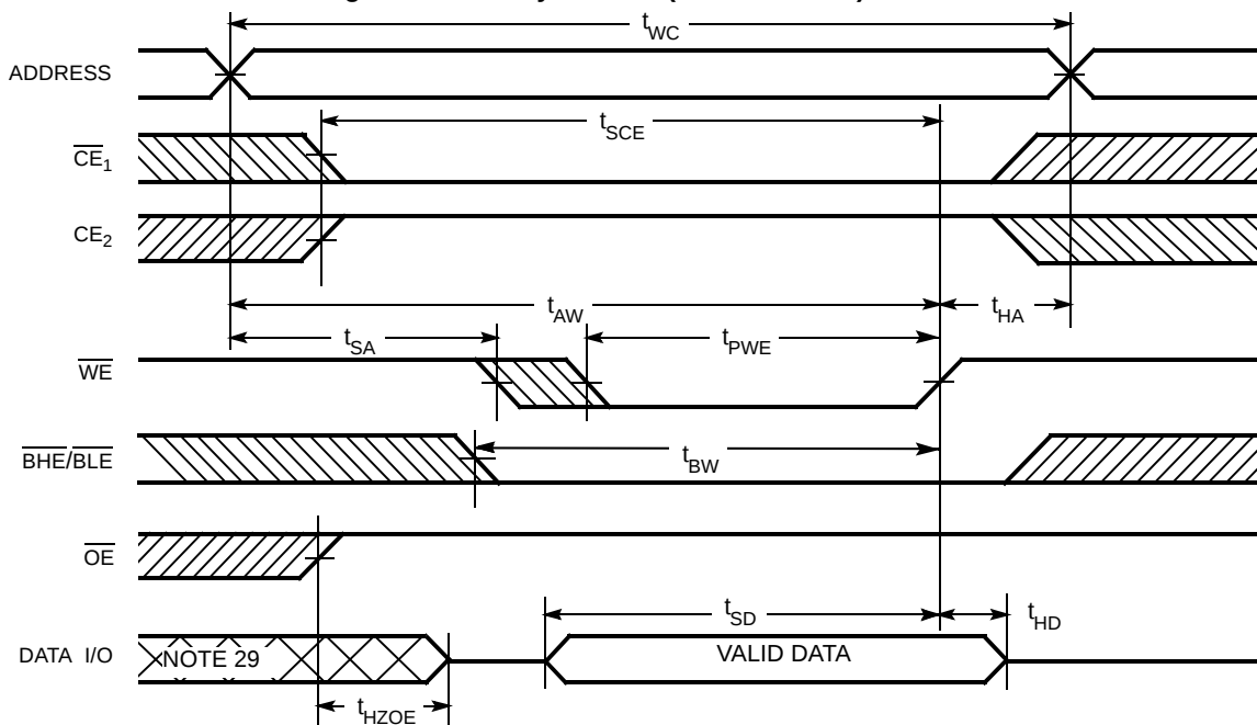
Figure 8. Write Cycle No. 2 ( \overline{\text{CE}}_1 or \text{CE}_2 Controlled) [26, 27, 28, 29]
