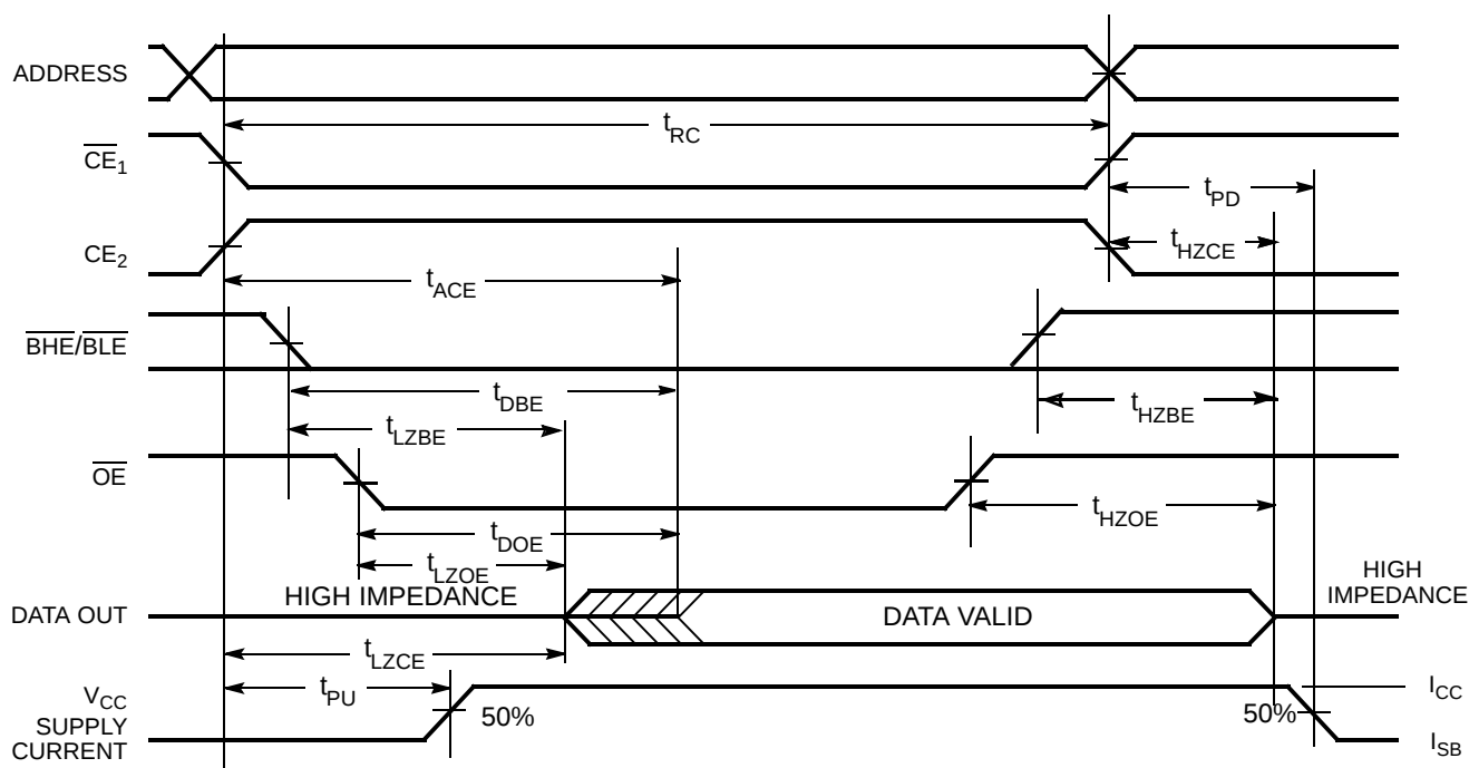
Figure 6. Read Cycle No. 2 ( \overline{\text{OE}} Controlled) [24, 25]
