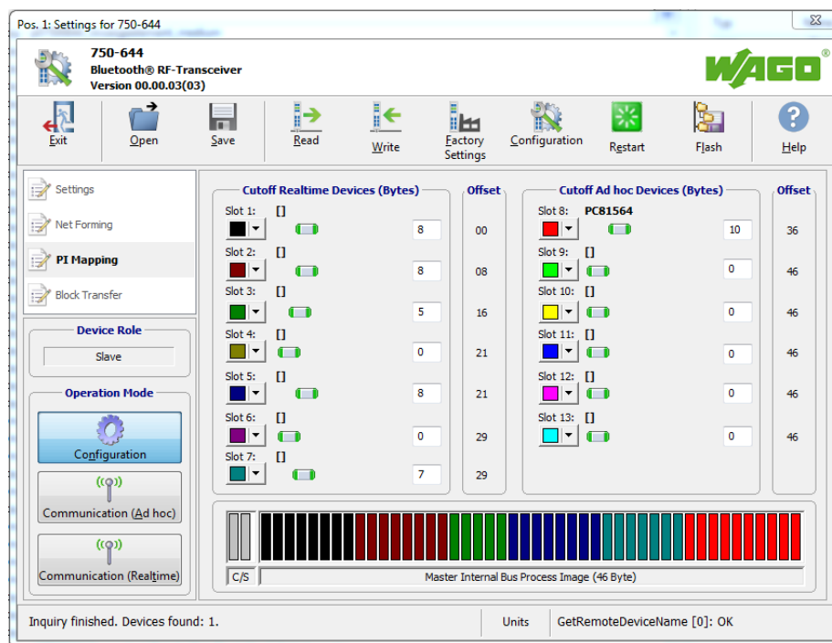
Figure 33: Screenshot of the PI Mapping page
