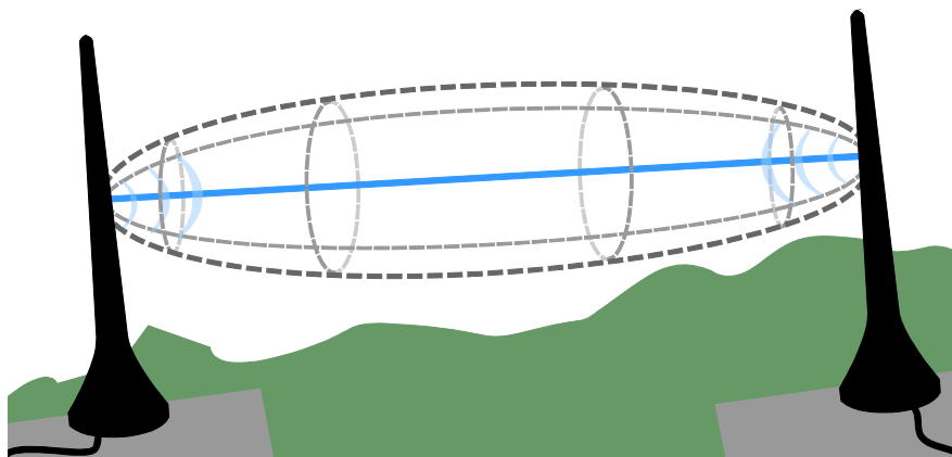
Figure 22: Fresnel zone
