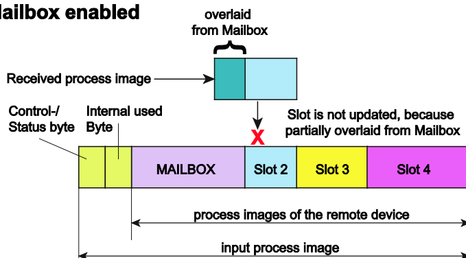
Figure 16: Partial overlay of process data by the Mailbox – PII
