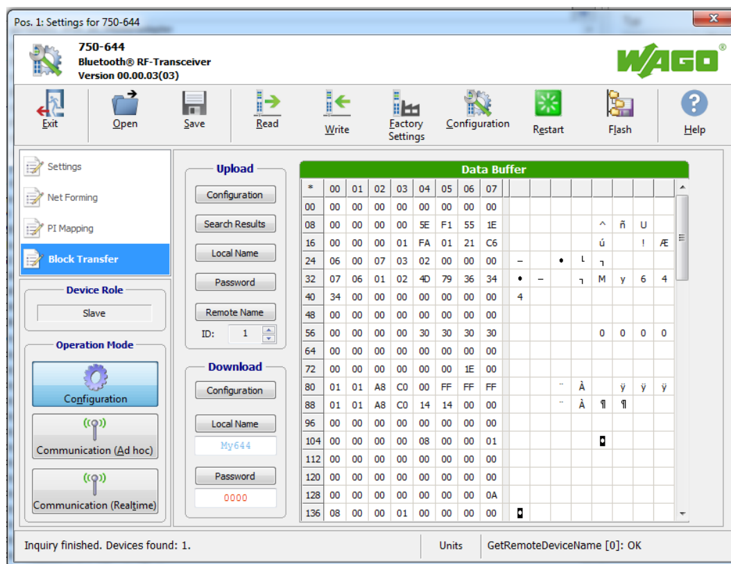
Figure 36: Screenshot of the Block Transfer page
