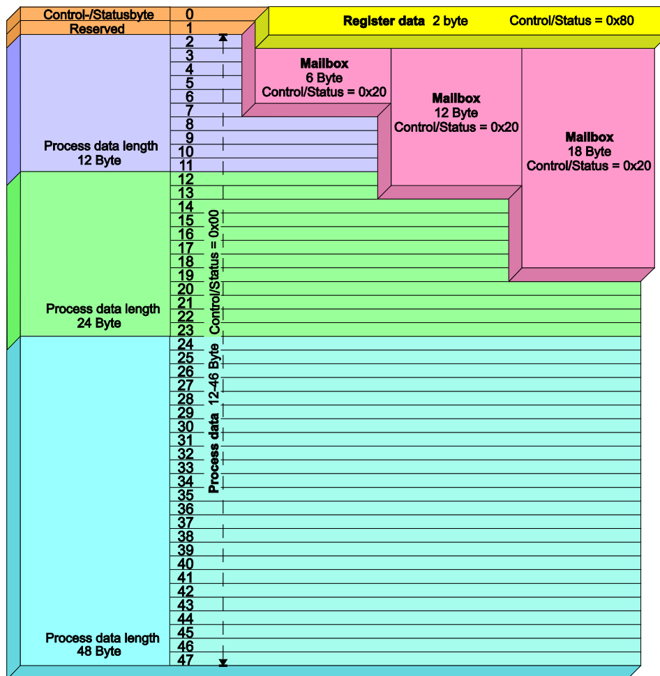
Figure 14: Process data overlaid with Mailbox or register data
