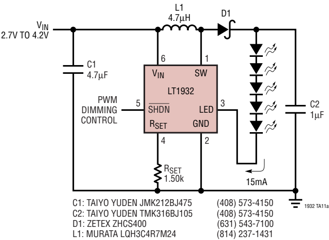
Li-Ion Driver for Five White LEDs
