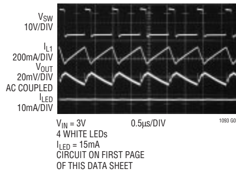
Switching Waveforms
