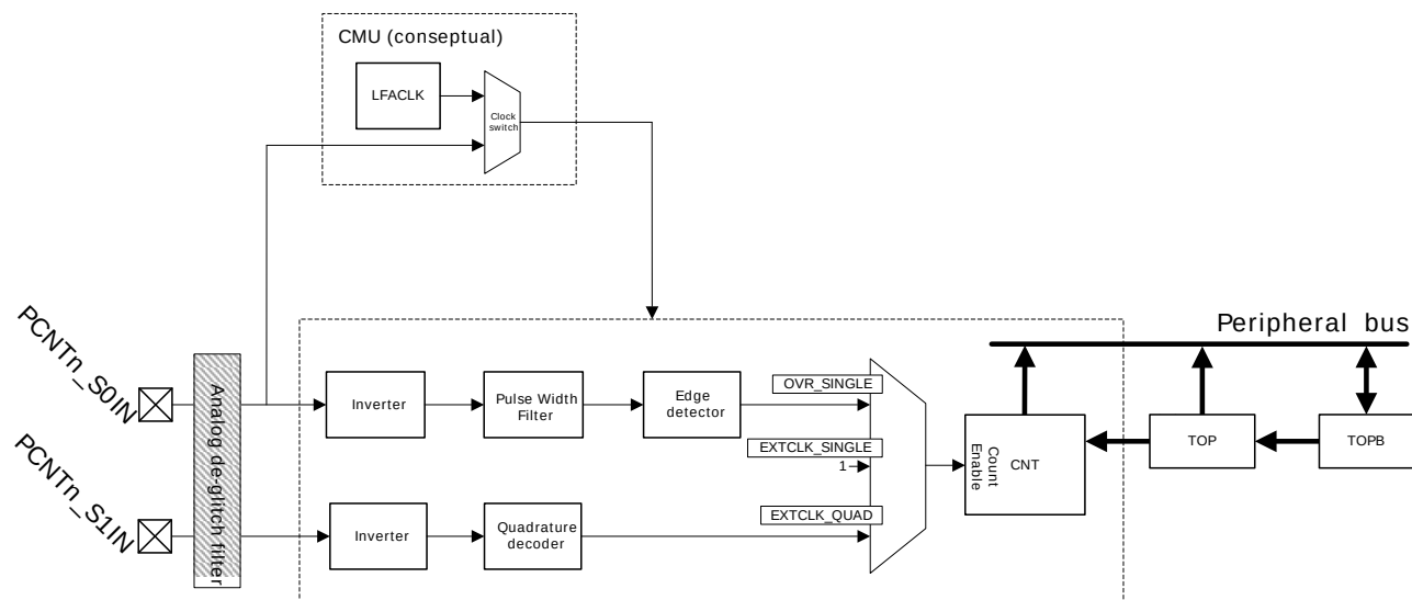
Figure 22.1. PCNT Overview
