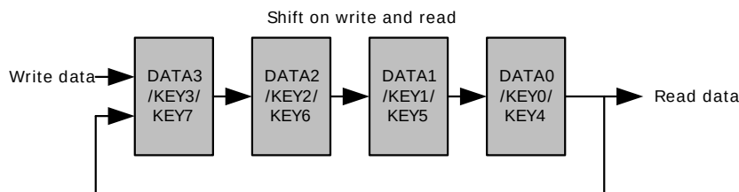
Figure 27.3. AES Data and Key Register Operation
