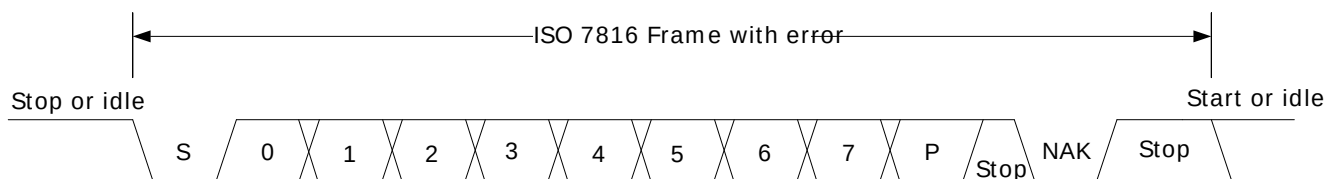
Figure 16.12. USART ISO 7816 Data Frame With Error
