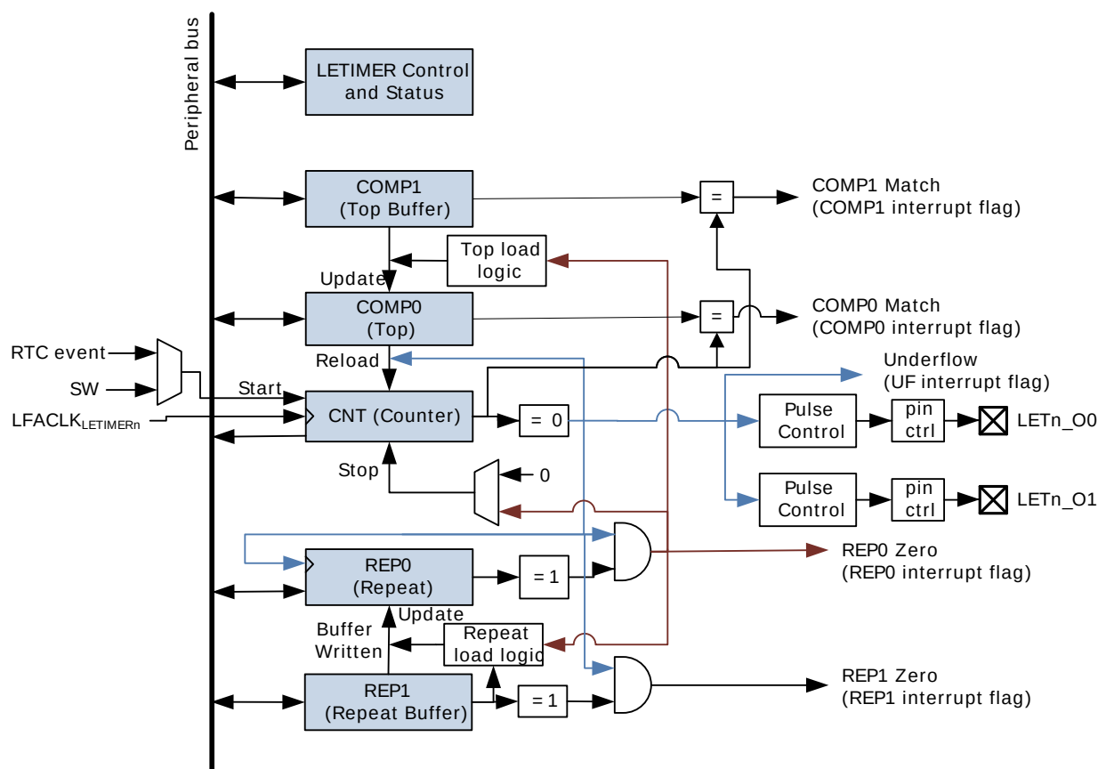
Figure 21.1. LETIMER Overview
