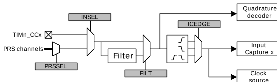
Figure 19.10. TIMER Input Pin Logic
