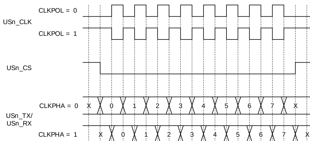
Figure 16.14. USART SPI Timing
