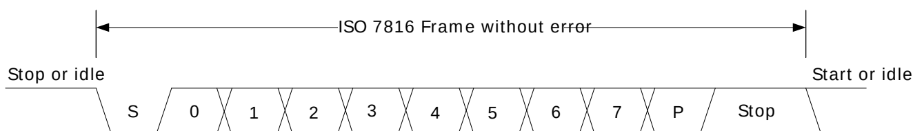
Figure 16.11. USART ISO 7816 Data Frame Without Error
