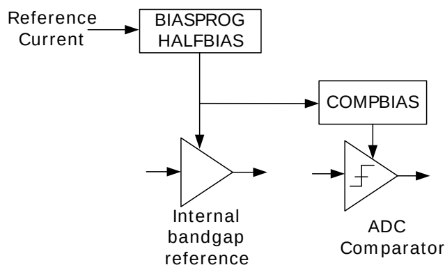
Figure 25.3. ADC Bias Programming
