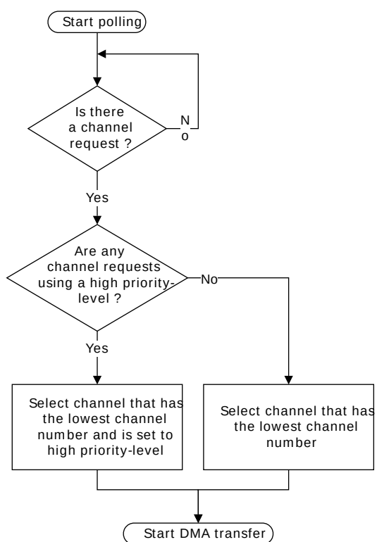
Figure 8.2. Polling flowchart
