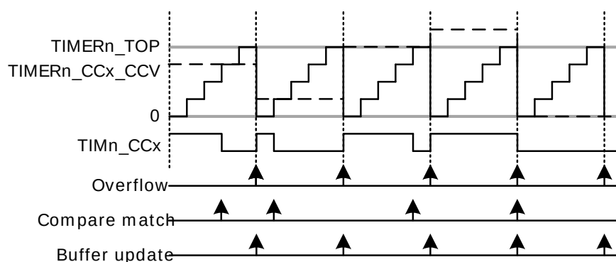
Figure 19.18. TIMER Up-count Frequency Generation
