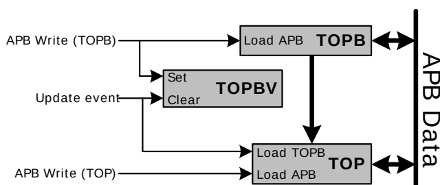
Figure 19.5. TIMER TOP Value Update Functionality
