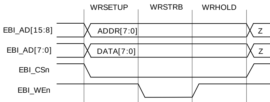
Figure 14.3. EBI 8-bit Write Operation
