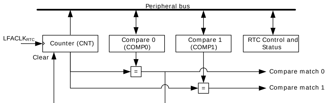
Figure 20.1. RTC Overview
