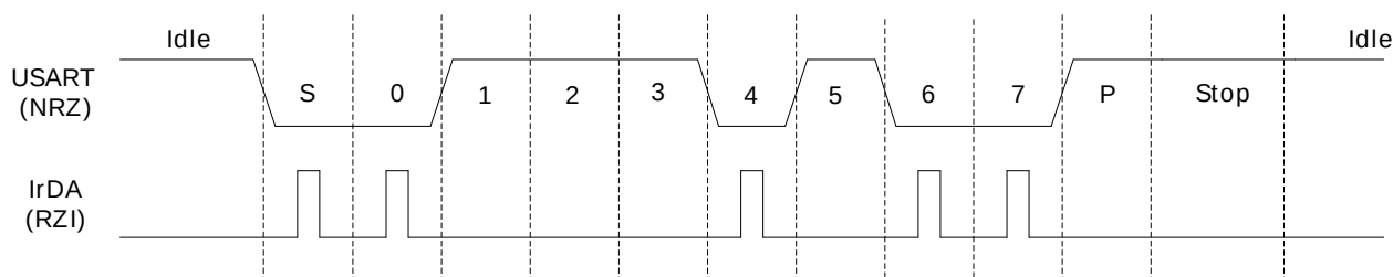
Figure 16.15. USART Example RZI Signal for a given Asynchronous USART Frame
