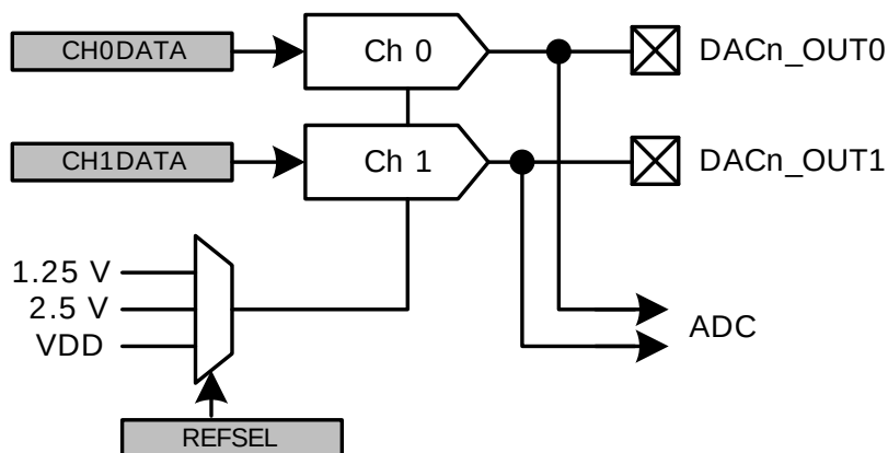
Figure 26.1. DAC Overview
