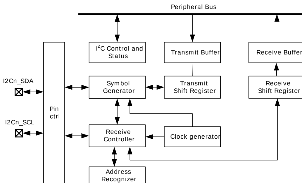
Figure 15.1. I 2 C Overview
