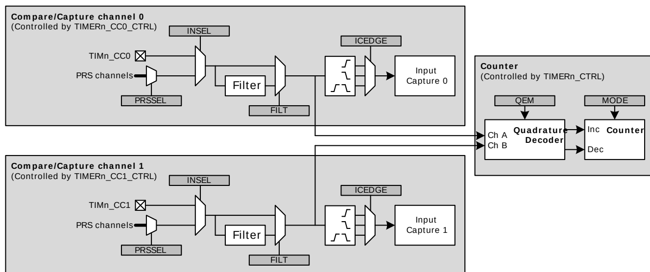
Figure 19.7. TIMER Quadrature Encoded Configuration
