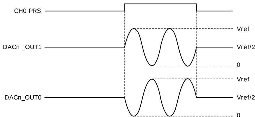
Figure 26.3. DAC Sine Mode
