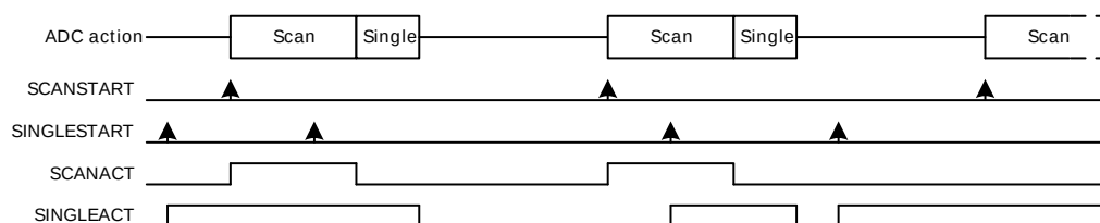
Figure 25.4. ADC Conversion Tailgating
