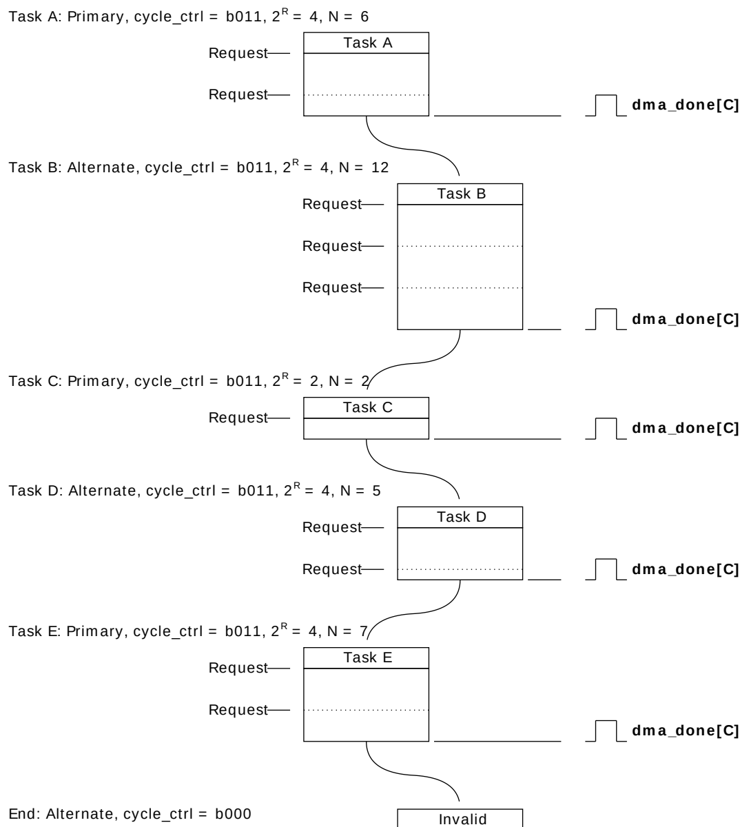
Figure 8.3. Ping-pong example
