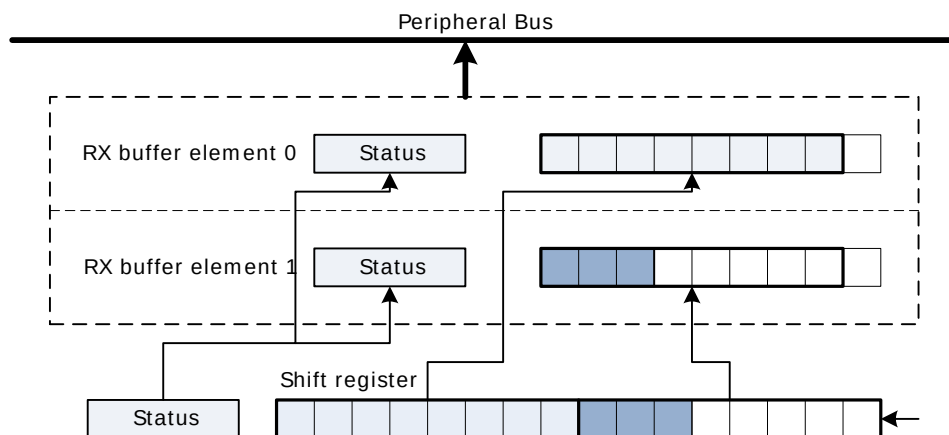
Figure 16.10. USART Reception of Large Frames
