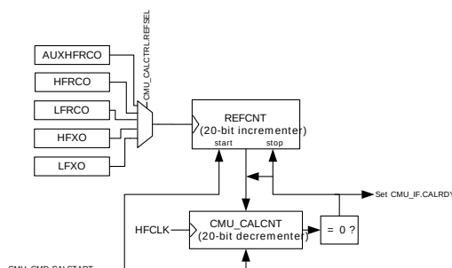
Figure 11.6. CMU Overview of the HW-support for RC Oscillator Calibration
