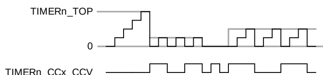
Figure 19.17. TIMER Up-count Frequency Generation
