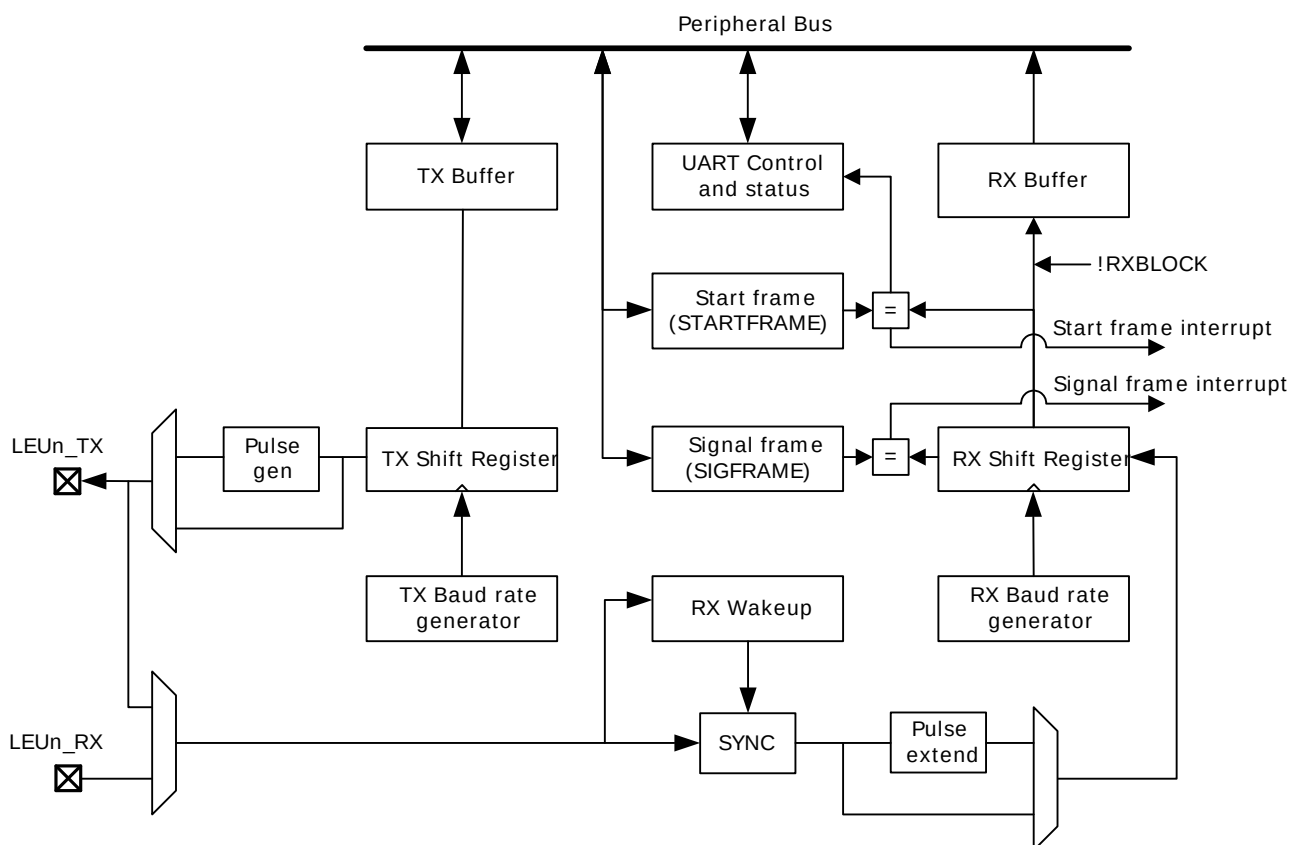
Figure 18.1. LEUART Overview
