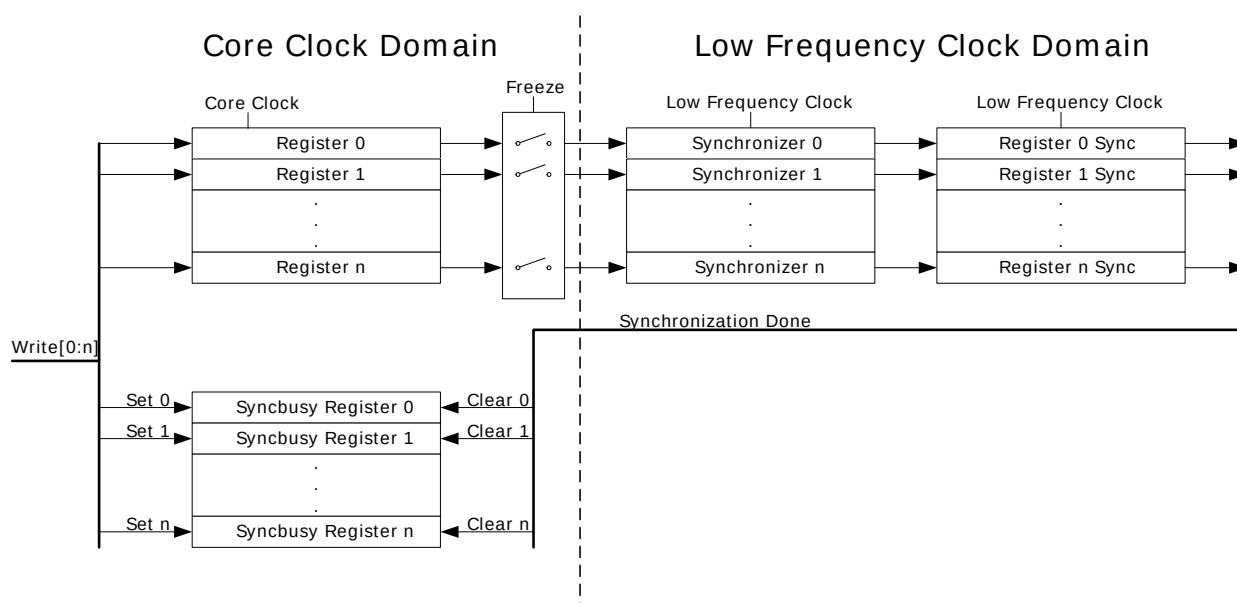
Figure 5.2. Write operation to Low Energy Peripherals
