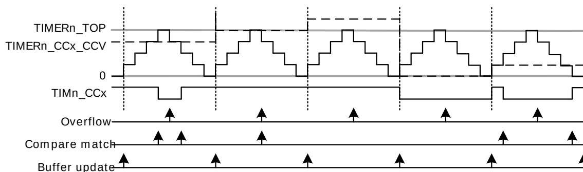
Figure 19.19. TIMER Up/Down-count Frequency Generation
