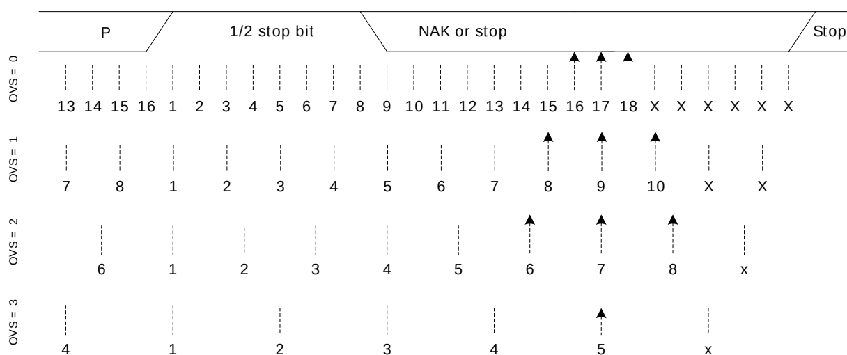
Figure 16.13. USART SmartCard Stop Bit Sampling
