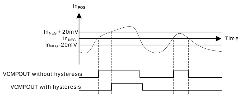
Figure 24.2. VCMP 20 mV Hysteresis Selected
