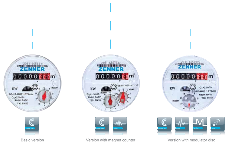
Single-jet meter ETKD/ETWD
