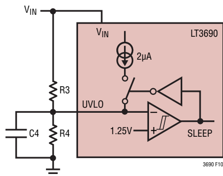
Figure 10. Undervoltage Lockout
