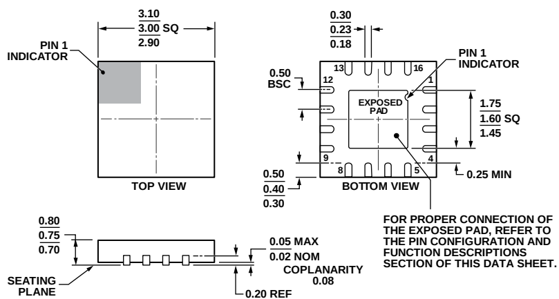
Figure 44. 16-Lead Lead Frame Chip Scale Package [LFCSP_WQ] 3 mm × 3 mm Body, Very Very Thin Quad (CP-16-22)
