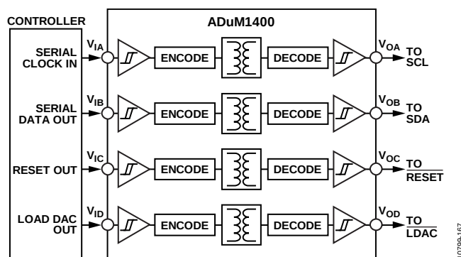
Figure 43. Isolated Interface
