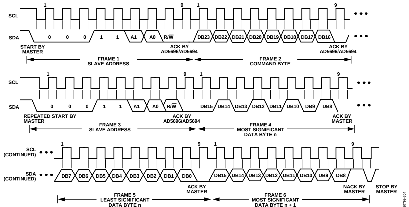
Figure 38. I²C Read Operation
