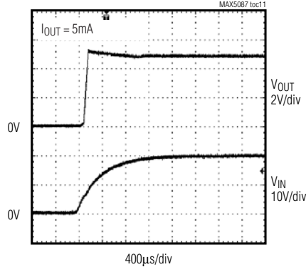
STARTUP RESPONSE
