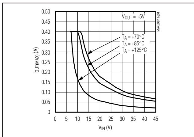
Figure 4. Maximum Output Current vs. Input Voltage (16-Pin TQFN)
