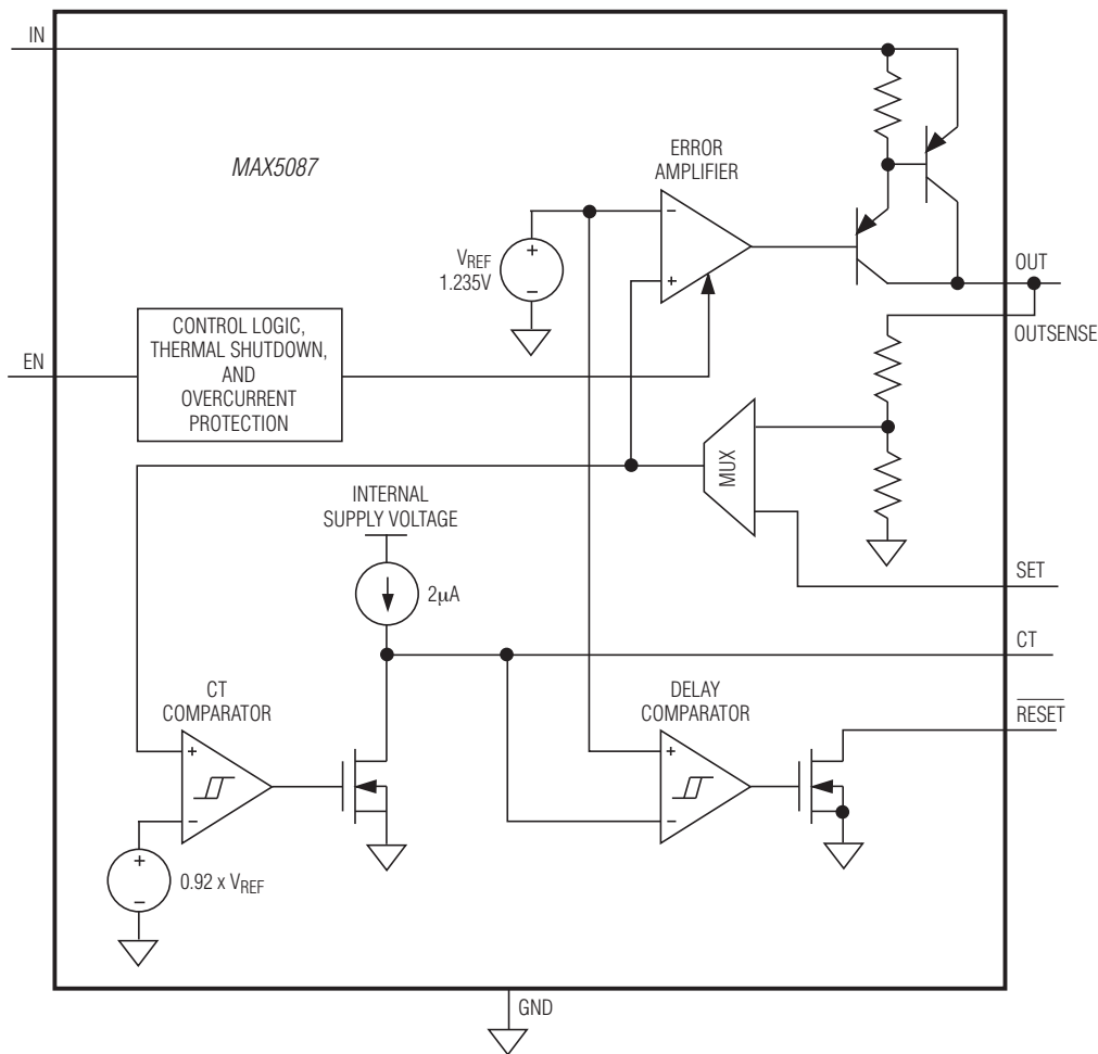
Figure 1. Functional Diagram
