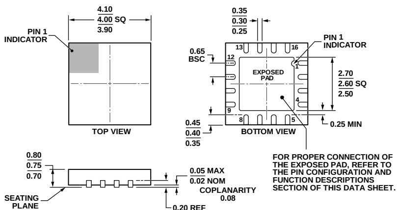
Figure 61. 16-Lead Lead Frame Chip Scale Package [LFCSP_WQ] 4 mm × 4 mm Body, Very Very Thin Quad (CP-16-17)
