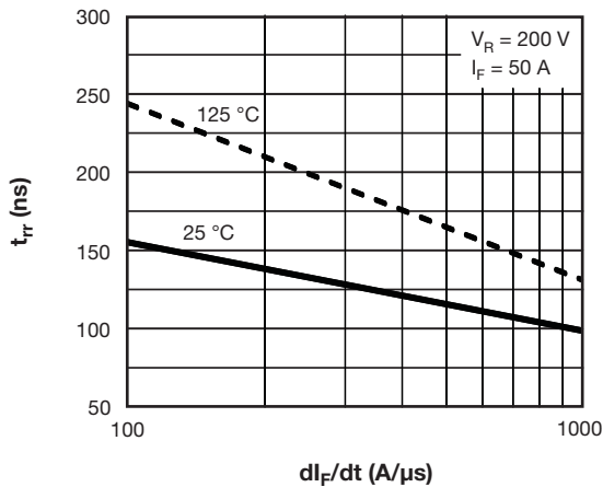
Fig. 13 - Typical t_r Diode vs. dI_F/dt V_{RR} = 200\text{ V} , I_F = 50\text{ A}
