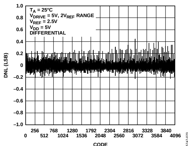
Figure 15. ADC DNL Differential, 2 \times V_{\text{REF}} Range
