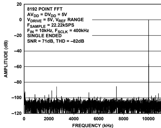
Figure 5. Signal-to-Noise Ratio Single-Ended, V REF Range
