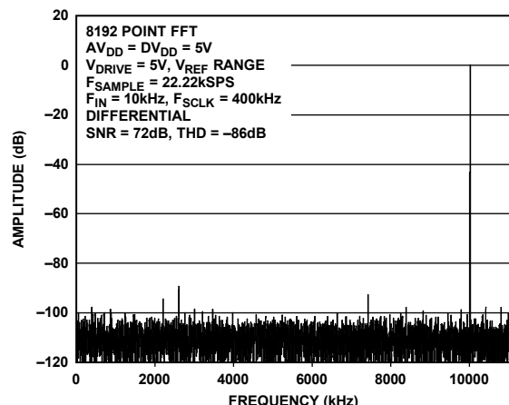
Figure 7. Signal-to-Noise Ratio Differential, V REF Range
