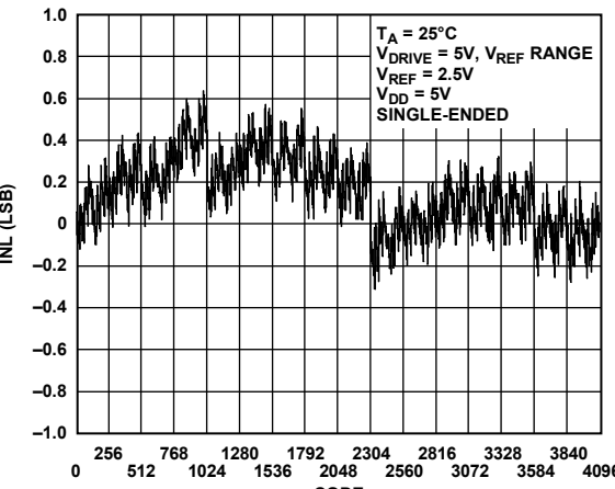
Figure 9. ADC INL Single-Ended, V REF Range
