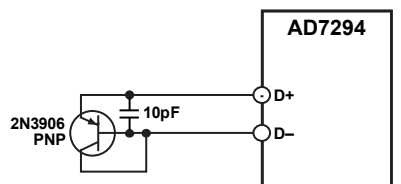
Figure 46. Measuring Temperature Using a PNP Transistor
