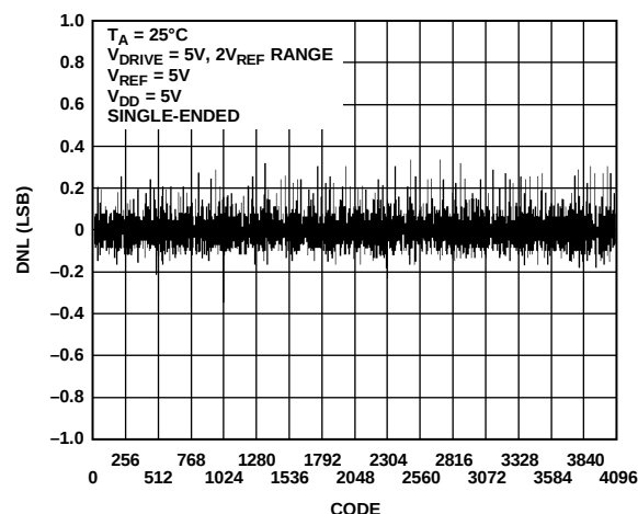
Figure 12. ADC DNL Single-Ended, 2 \times V_{\text{REF}} Range
