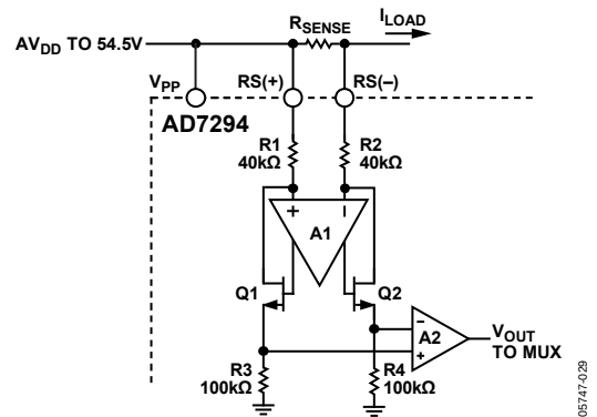
Figure 41. High-Side Current Sense
