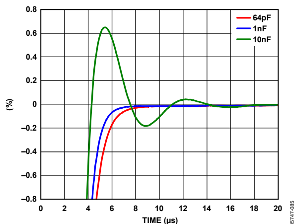
Figure 23. Zoomed in Settling for a \frac{1}{4} to \frac{3}{4} Output Voltage Step
