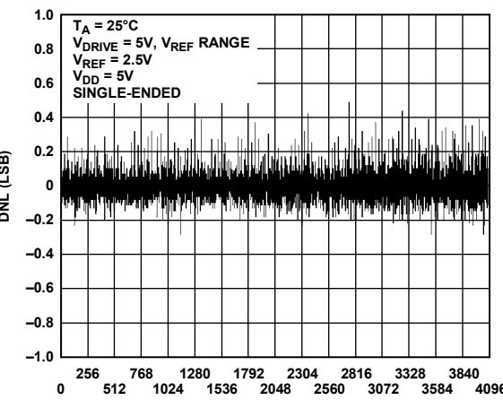
Figure 10. ADC DNL Single-Ended, V REF Range
