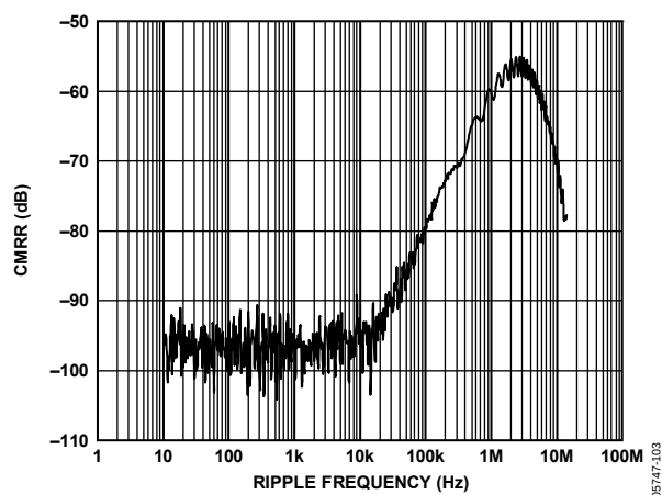
Figure 33. I_{\text{SENSE}} Common-Mode Rejection Ratio vs. Ripple Frequency for a 400 mV Peak-To-Peak Ripple
