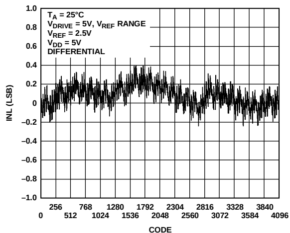
Figure 13. ADC INL Differential, V_{\text{REF}} Range
