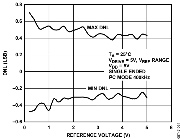
Figure 18. ADC DNL vs. Reference Voltage
