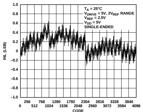
Figure 11. ADC INL Single-Ended, 2 \times V_{\text{REF}} Range
