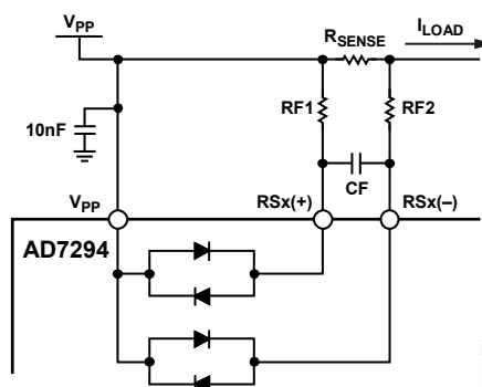
Figure 42. Current Sense Filtering ( RS_X Can Be Either RS1 or RS2)
