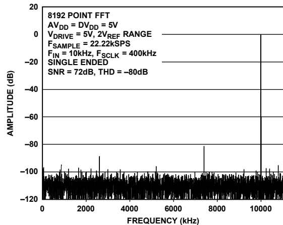
Figure 6. Signal-to-Noise Ratio Single-Ended, 2 × V REF Range
