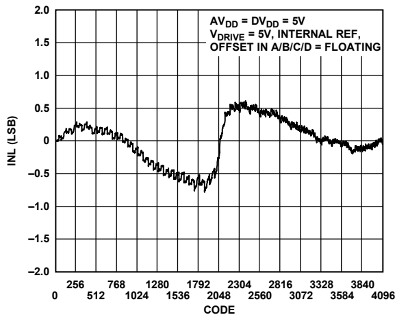
Figure 19. DAC INL
