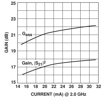
Figure 14. Gain, |S_{21}|^2 , and Gain Associated with Minimum Noise vs. Current.
