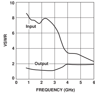
Figure 13. Input and Output VSWR vs. Frequency.
