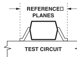
Figure 25. Phase Reference Planes.
