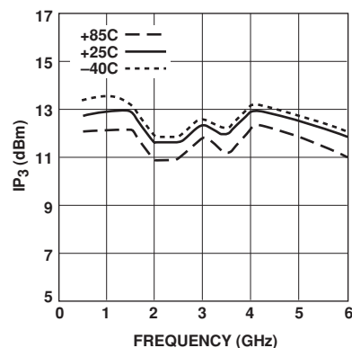
Figure 9. Output Third Order Intercept Point vs. Frequency and Temperature.
