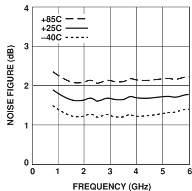
Figure 3. Minimum Noise Figure vs. Frequency and Temperature.
