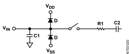
Figure 18. Equivalent Analog Input Structure
