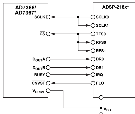
Figure 29. Interfacing the AD7366/AD7367 to the ADSP-218x
