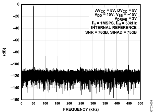
Figure 5. AD7367 FFT
