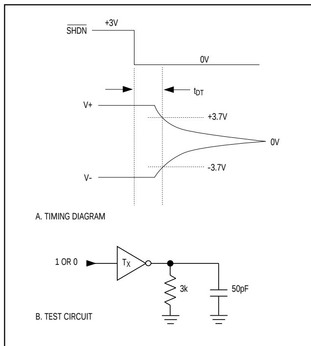
Figure 5. Transmitter Output Disable Timing
