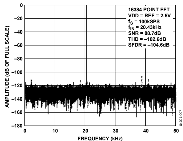
Figure 12. FFT Plot
